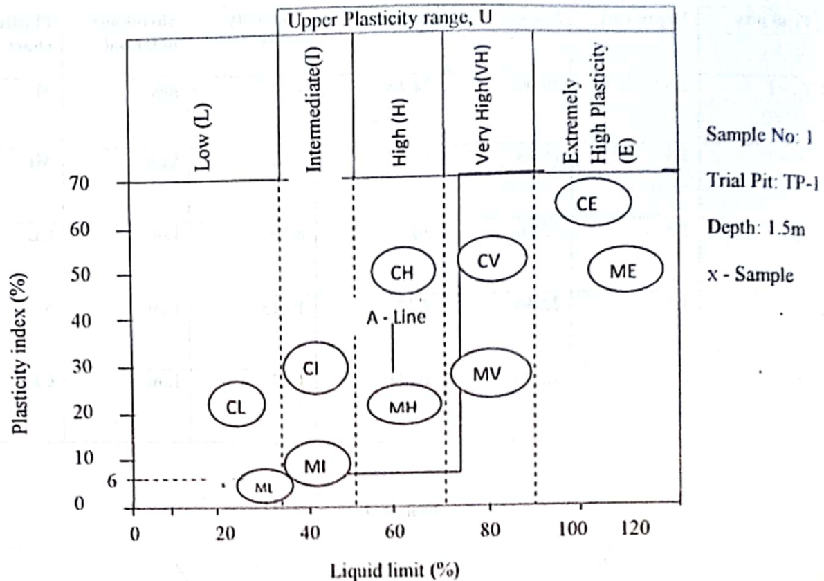
Figure 8: Plot of Plasticity Index (PI) against Liquid Limit (LL)
