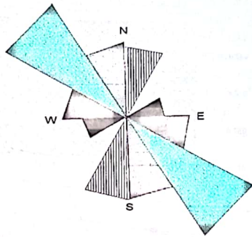
Figure 3: Rosette diagram (Omanayin, 2008)
