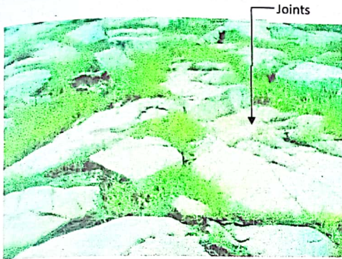
Plate 1: An outcrop with joints (Omanayin, 2008)
