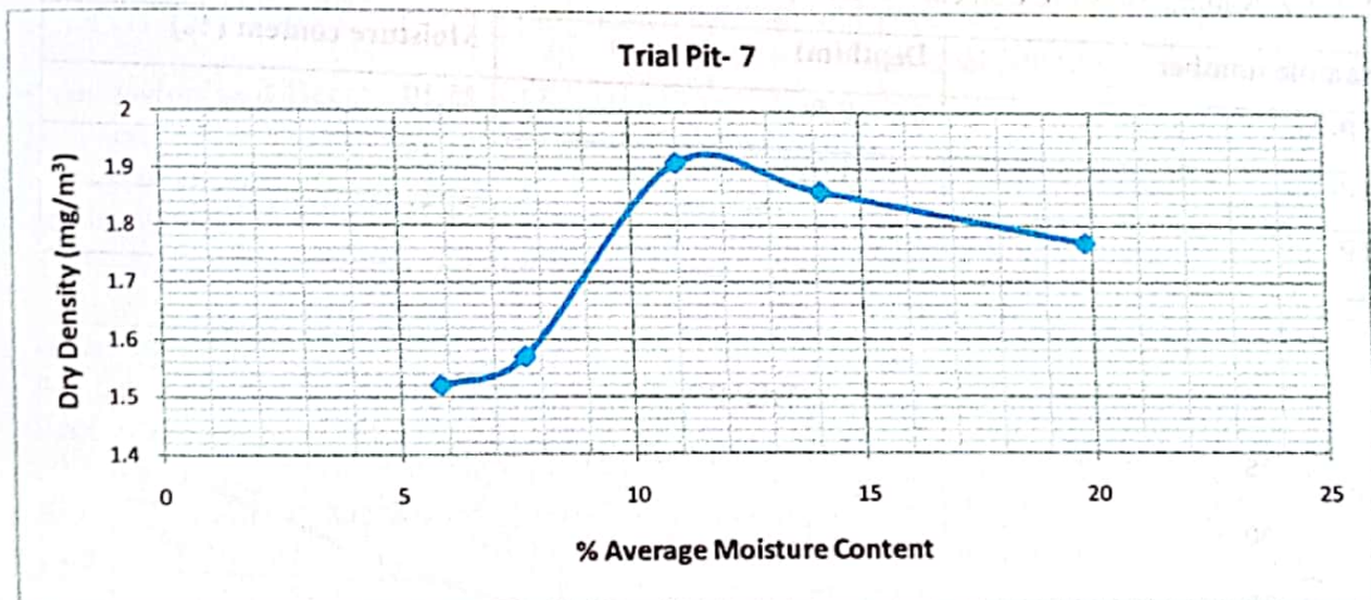
Figure 9: Compaction graph of trial pit- 7
