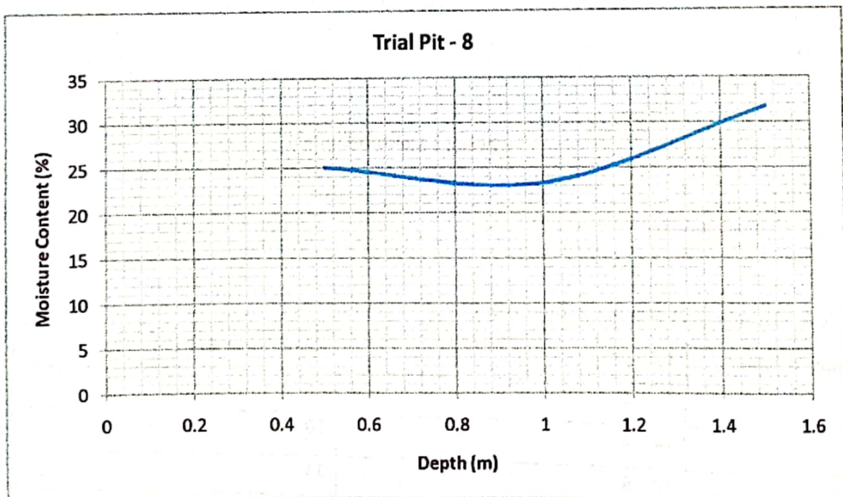
Figure 10: Natural Moisture Content graph of Trial pit-8
