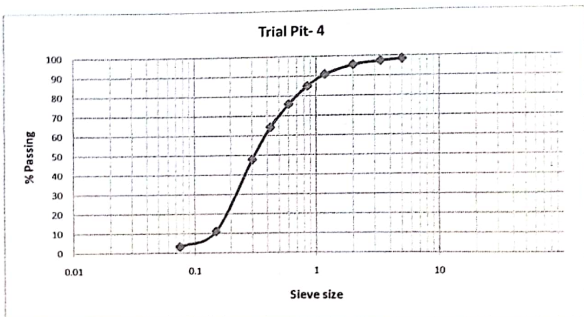
Figure 6: A representative soil particle distribution curve from the study area
