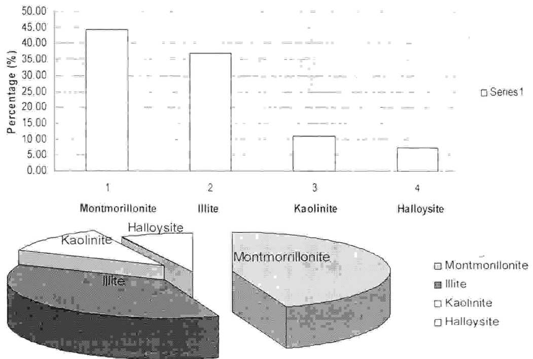
Fig. 8. Pie-chart of inferred clay minerals
