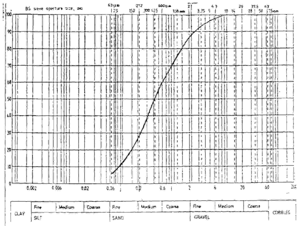
Fig. 5. A typical particle distribution curve from the study area
