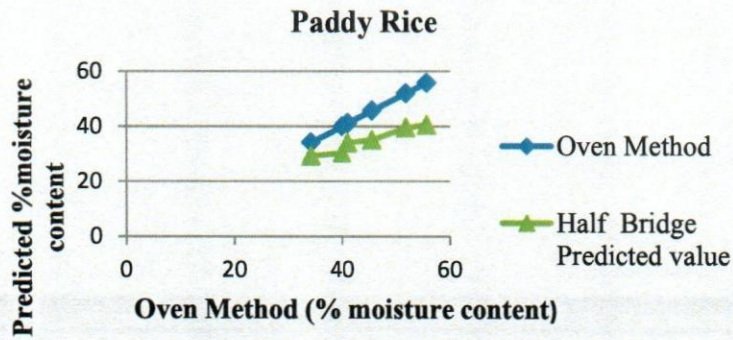
Figure 5: Predicted %moisture content of Paddy rice versus Oven Method
