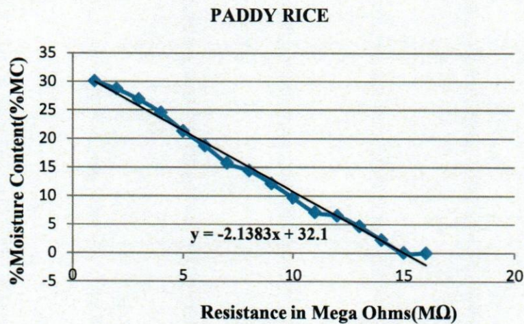
Figure 2: %Moisture Content versus Measured Resistance of Rice
