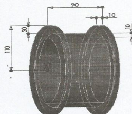
Figure 3: Showing the fully revolved sketched rim
