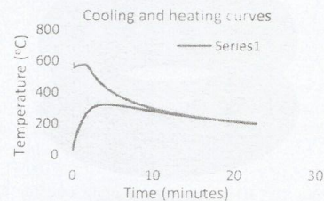
Figure 18: Comparison of the cast and mould temperatures
