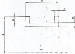
Figure 1: The sketch of half rim
