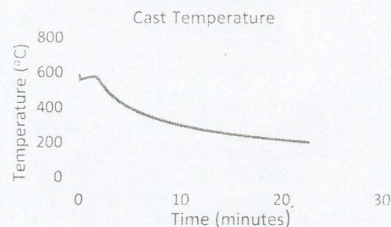
Figure 16: Graph showing casting temperature with time (cooling curve)
