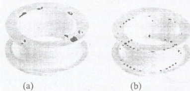
Figure 14: 3D plot of hot spots based on (a) solidification time for the initial simulation, (b) Critical Fraction Solid Time for the initial simulation
