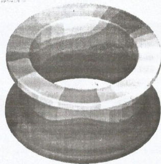
Figure 6: 3D plot of the solidification time for the initial simulation
