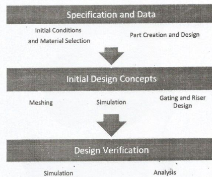
Figure 4: Sequence of the simulation process
