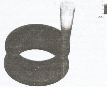
Figure 7: 3D plot of the solidification time for the final simulation
