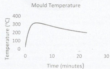
Figure 17: Graph showing mould temperature with time
