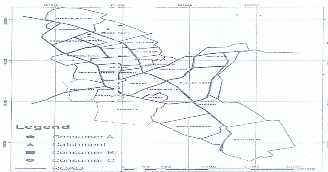
Figure 1: Map showing sample locations in Bosso area
