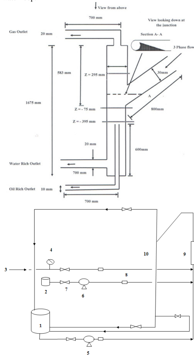
Figure 3.8: Diagram of the Air-Water-Oil Separation Experimental Flow Loop
