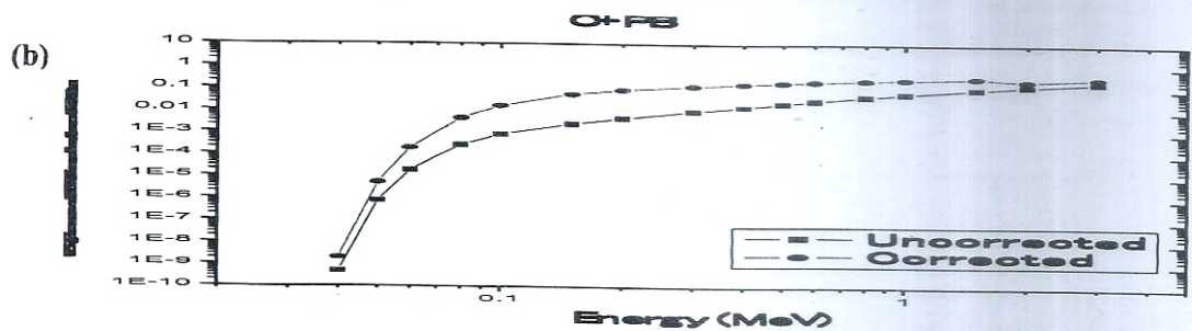
Figure 6: Exposure Buildup factors of various composite walls and concrete
