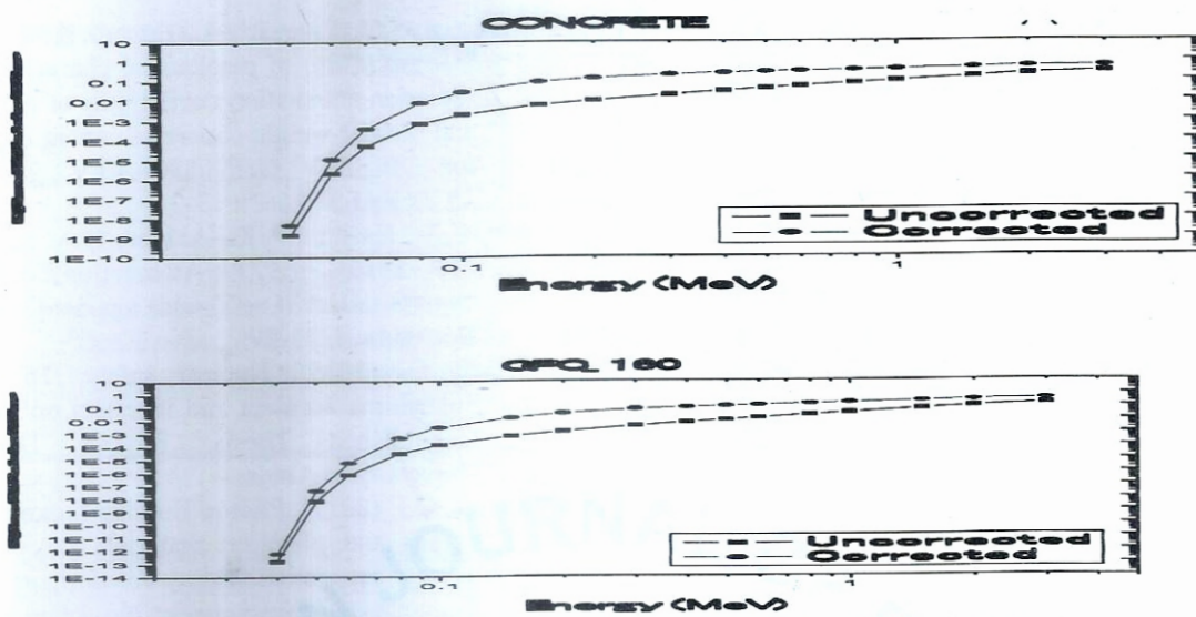
Figure 7: Corrected and uncorrected transmission factors of (a) GPC_160 ((b) C+PB (C) Concrete
