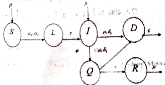
Fig.1.1 Schematic diagram of Ebola Fever transmission and Control model.
