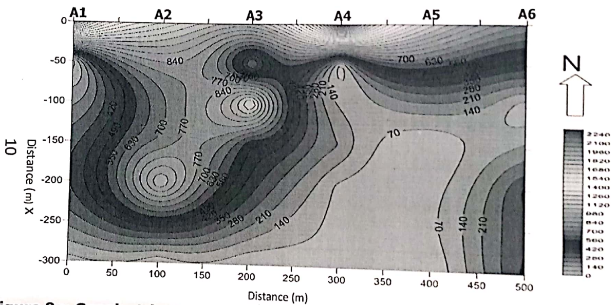
Figure 8a: Geoelectric Vertical section along Profile A (Contour Interval is 70? m)
