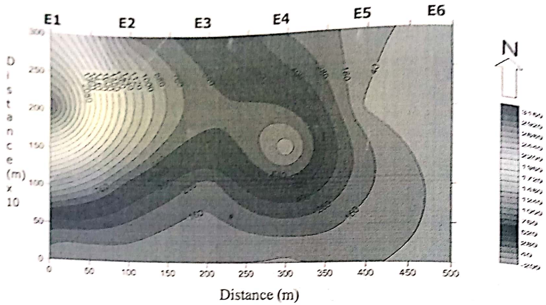
Figure 12a: Geoelectric Vertical Section along Profile E (Contour Interval is 120Ωm)
