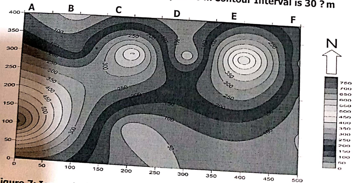
Figure 7: Iso-resistivity contour Map at 20 m Contour Interval is 50 ? m
