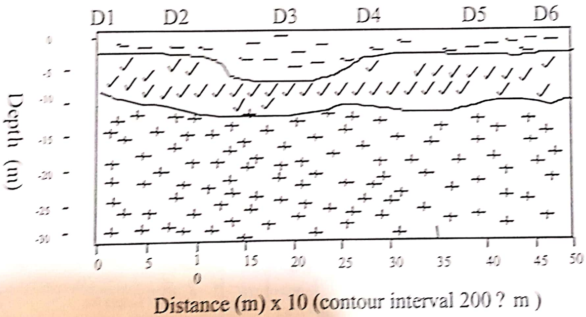
Figure 11b: Vertical Section through Profile D
