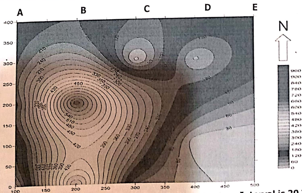
Figure 4: Iso-resistivity contour Map at Surface Contour Interval is 20 ? m
