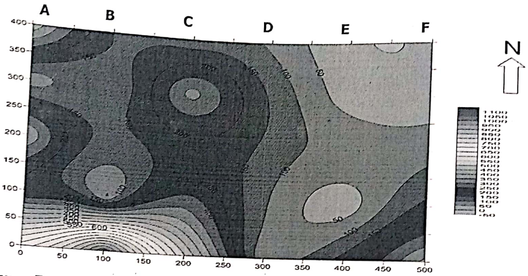
Figure 5: Iso-resistivity contour map at 5 m Contour Interval is 50 ? m
