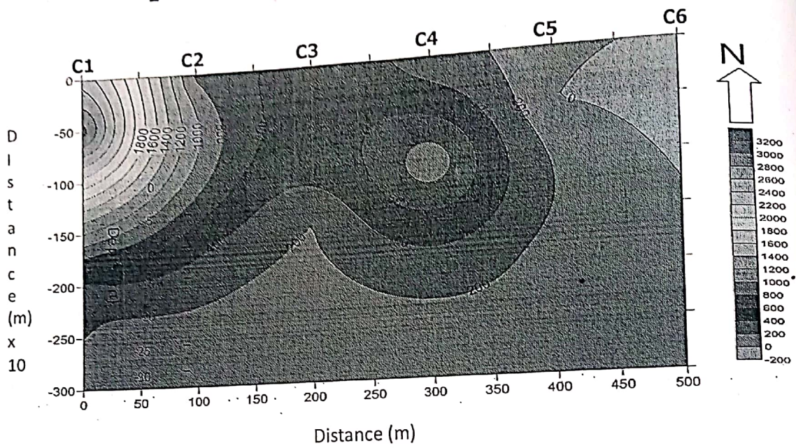
Figure 10a: Geoelectric Vertical section along
