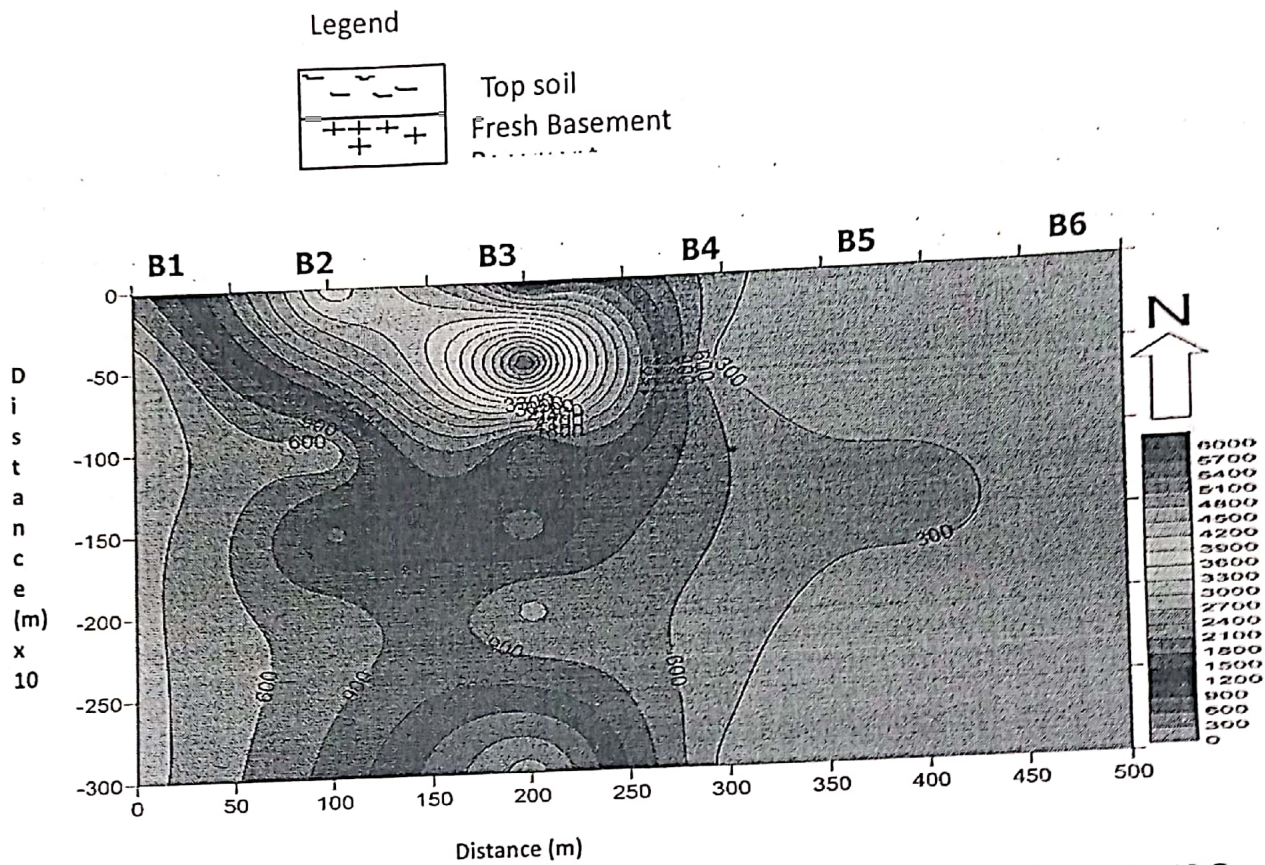
Figure 9a: Geoelectric Vertical section along Profile A (Contour Interval is 70 ? m)
