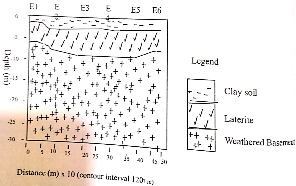
Figure 12b: Vertical Section through Profile
