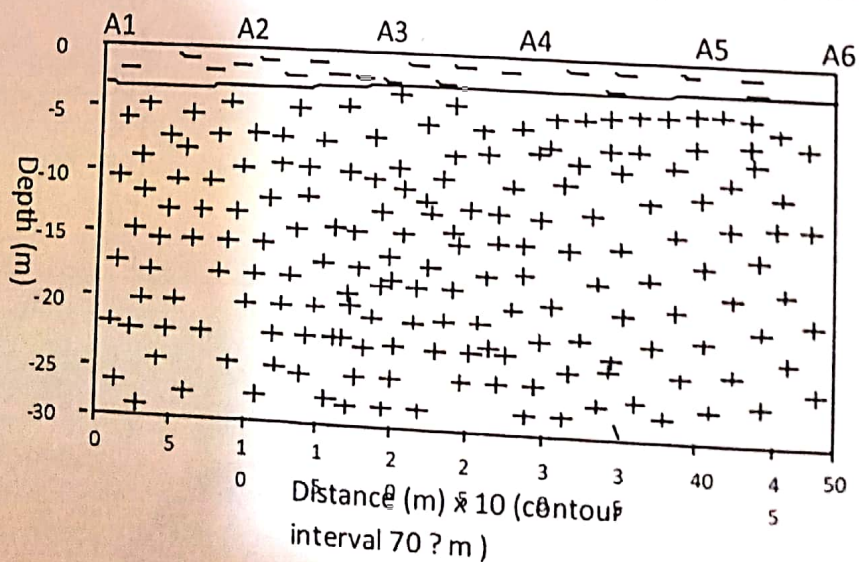
Figure 8b: Vertical Section through Profile A
