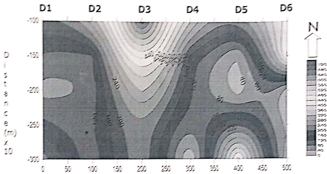
Figure 11a: Geoelectric Vertical section along Profile D (Contour Interval is 300?m)
