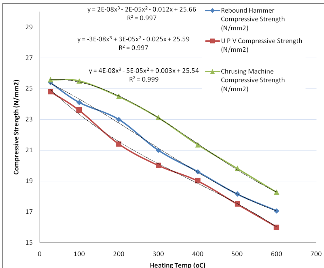
Figure 3 Compressive strength against heating temperature
