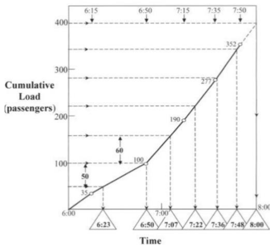
Figure 3: Determination of departure times with even load
