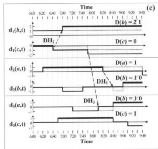
Figure 7. Network, schedule and DFs of the example
