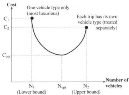
Figure 6. Optimization framework
