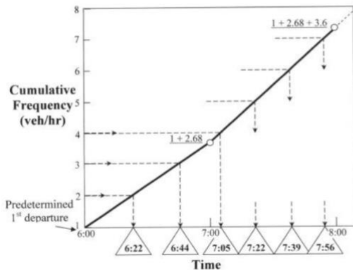
Figure 2: Determination of evenly spaced headways
