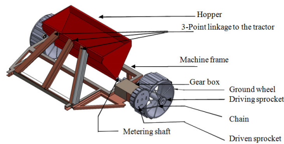
Figure 2. Auto CAD drawing of the equipment.
