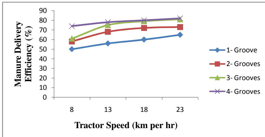
Figure 6. The relationship between uniformity in manure spreading and Tractor/Machine speed at 8% moisture content.
