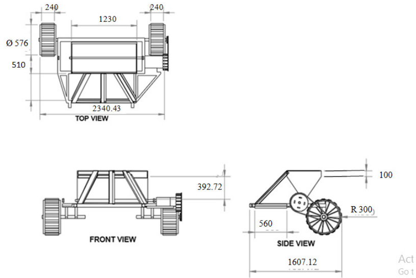
Figure 1. Orthographic projection of the equipment.
