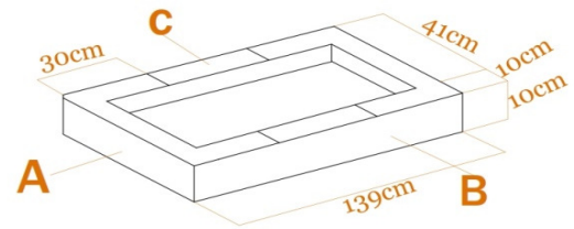
Figure 5. Sketch of the frame
