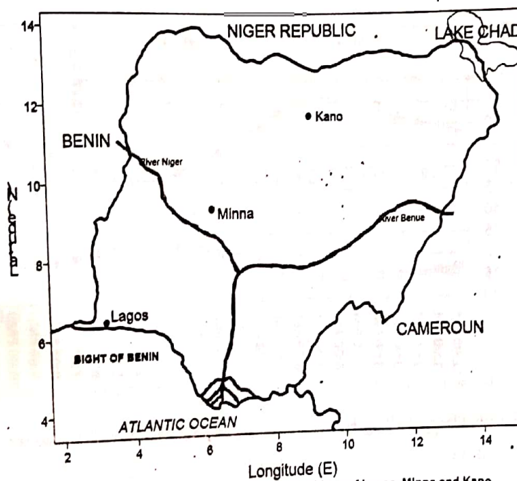
Fig. 1: Map of Nigeria Showing Relative Positions of Lagos, Minna and Kano
