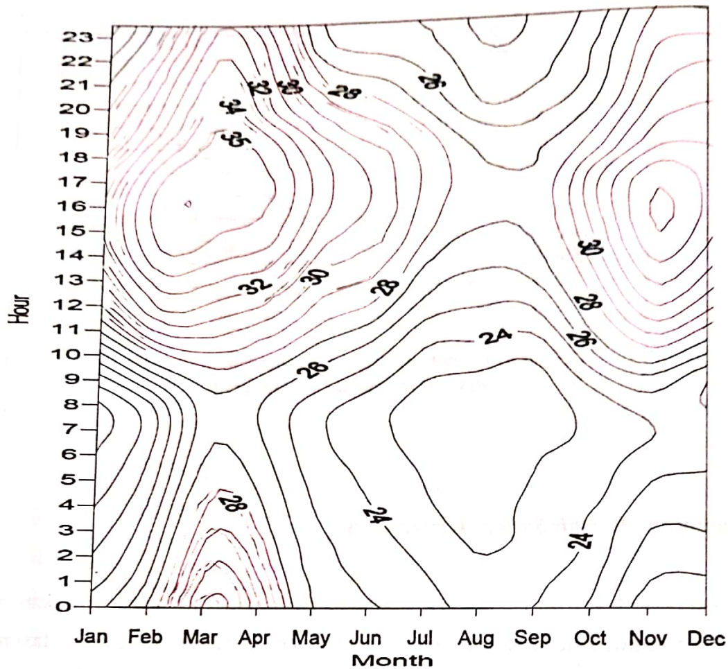
Figure 5: Mean Diurnal and Monthly Temperatures in Minna
