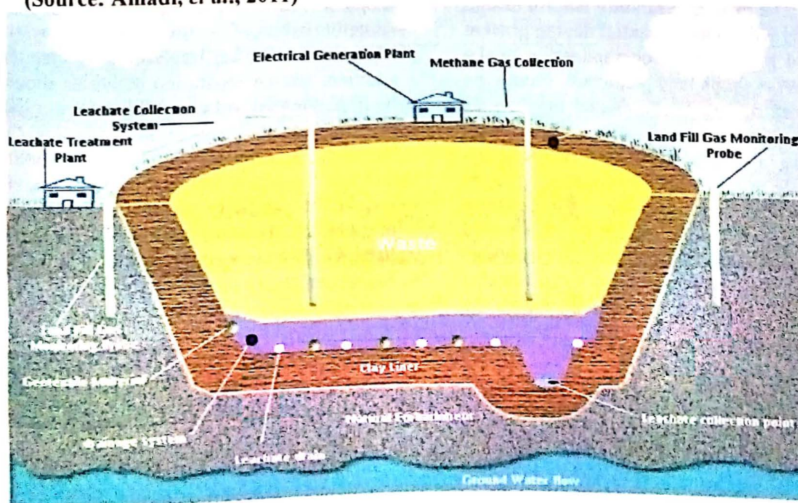
Fig. 3: A modern sanitary landfill with one clay liner for moderate vulnerability area (Source: Amadi, 2011)
