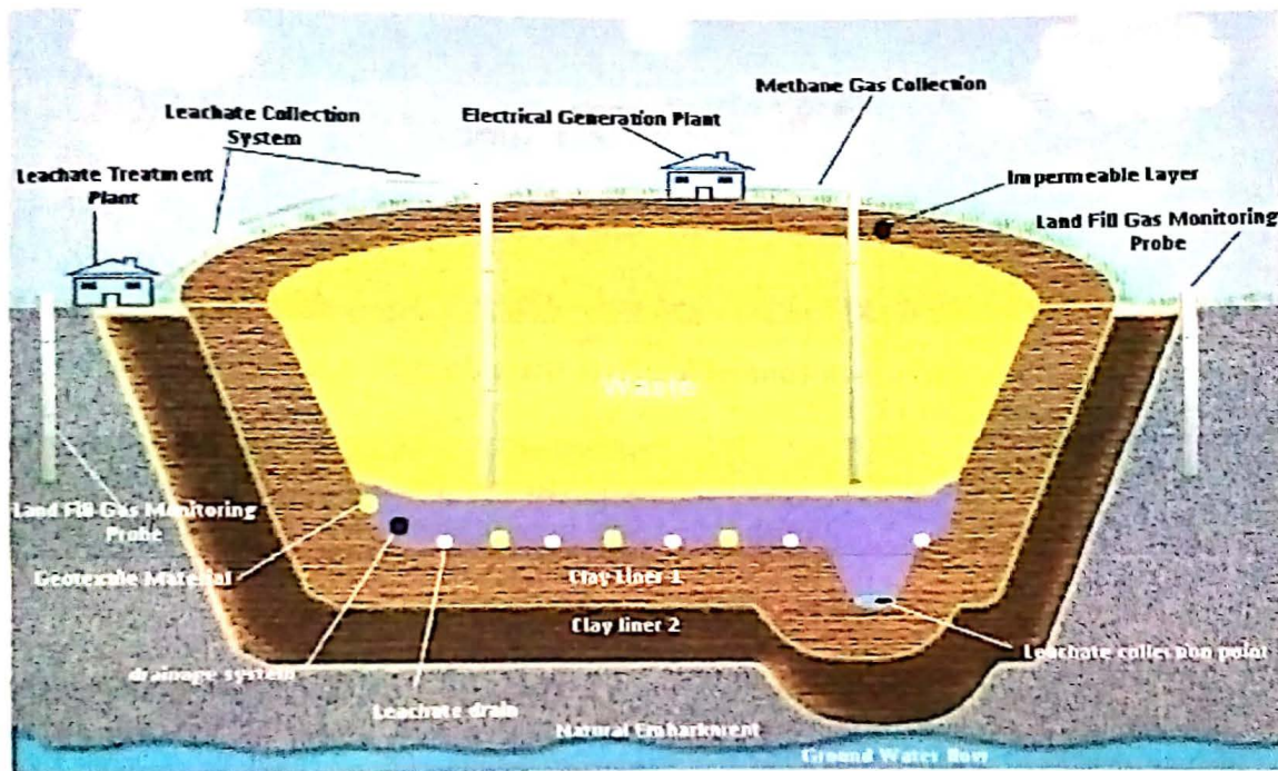
Fig.2: A modern sanitary landfill with two clay liners for high vulnerability area (Source: Amadi, et al. , 2011)
