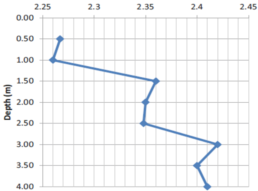
Fig. 6. Variation of Maximum Dry Density with depth
