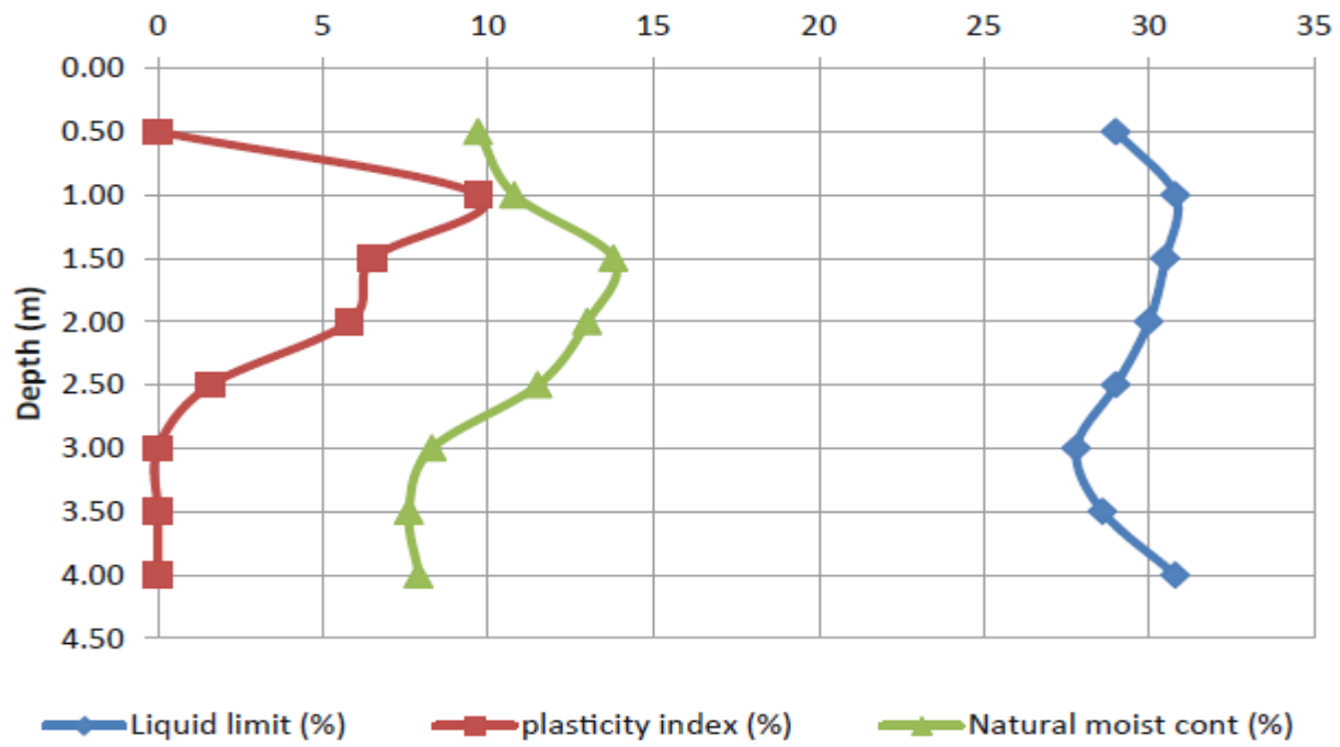
Fig. 4. Variation of Atterberg limit and NMC with depth
