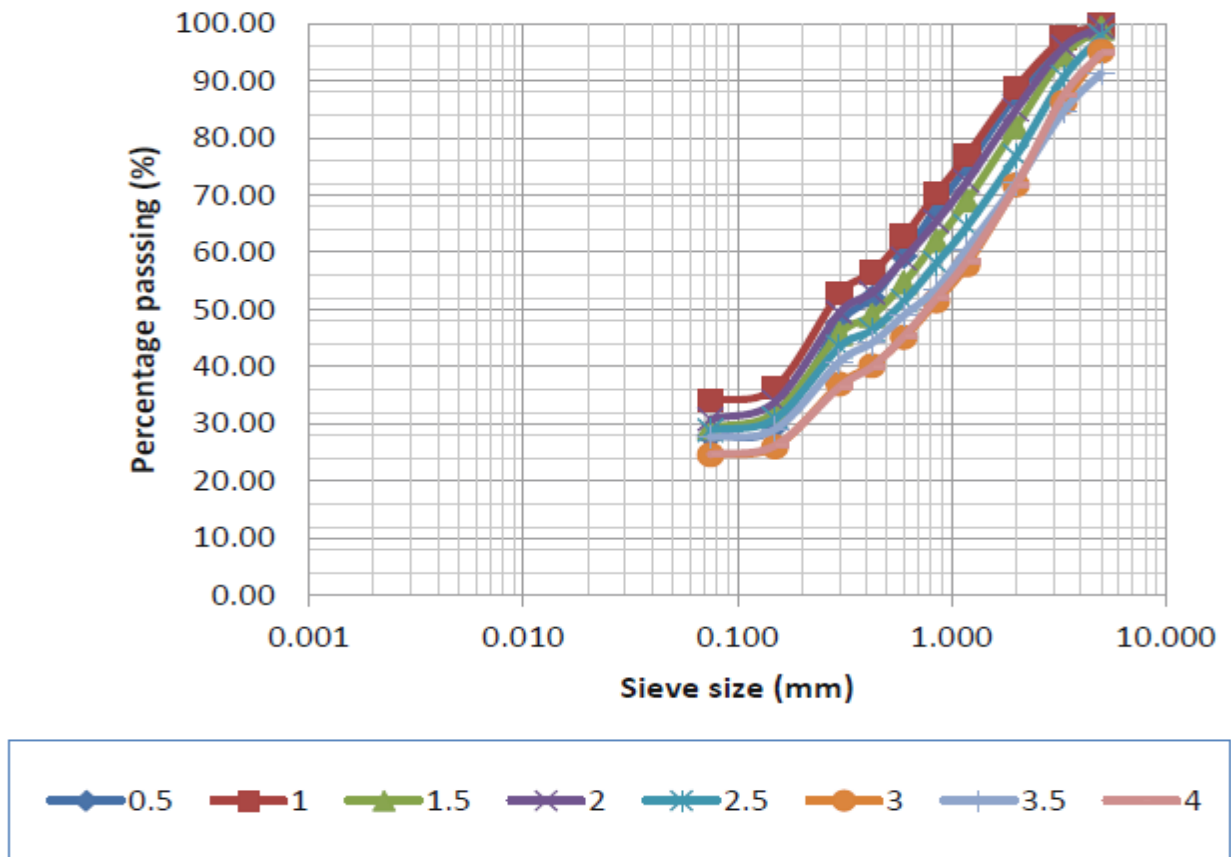
Fig. 5. Grain size analysis of soils within the profile
