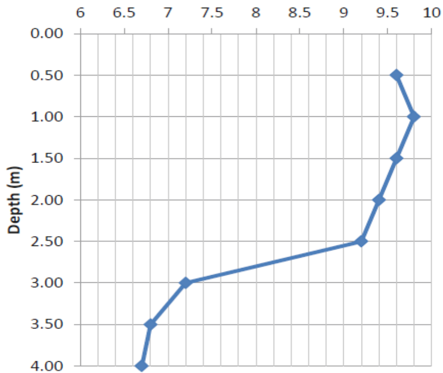
Fig. 7. Variation of Optimum Moisture Content with depth
