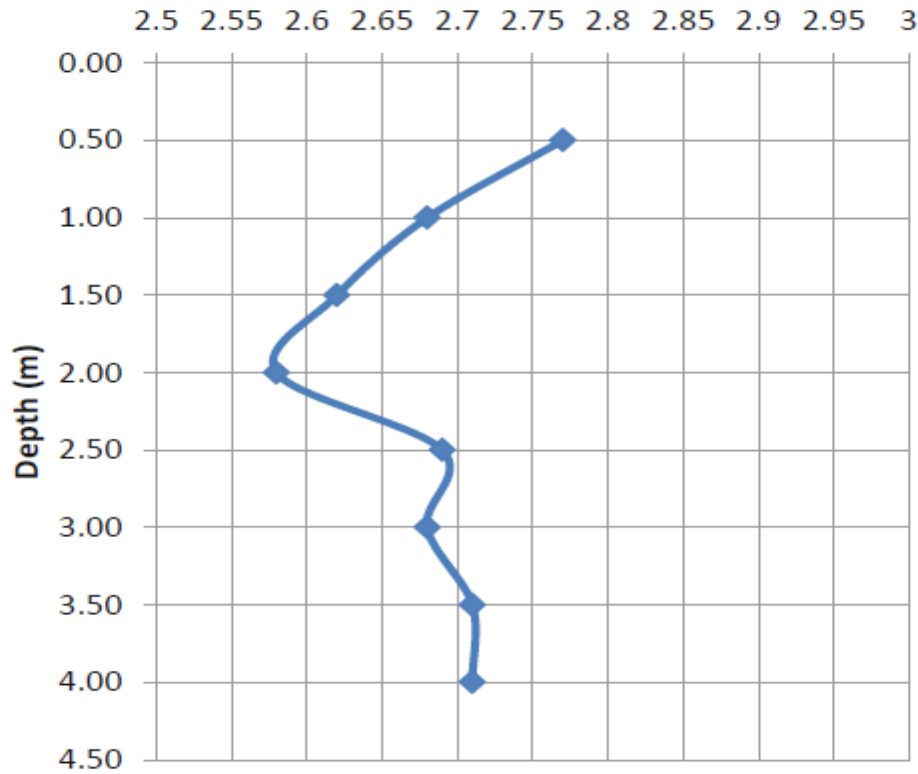
Fig. 8. Variation of specific gravity with depth
