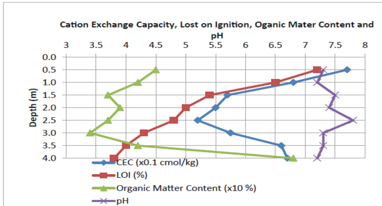
Fig. 3. Variation of physiochemical properties with depth
