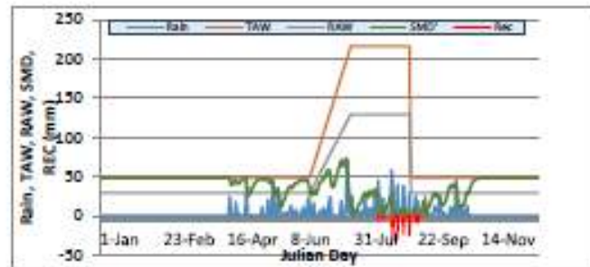
Figure 5: Soil Moisture Balance Components for 2010-Water year
