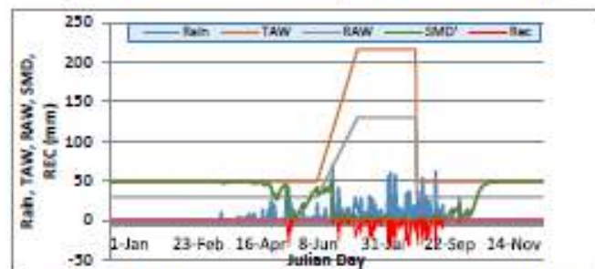
Figure 6: Soil Moisture Balance Components for 2012-Water year
