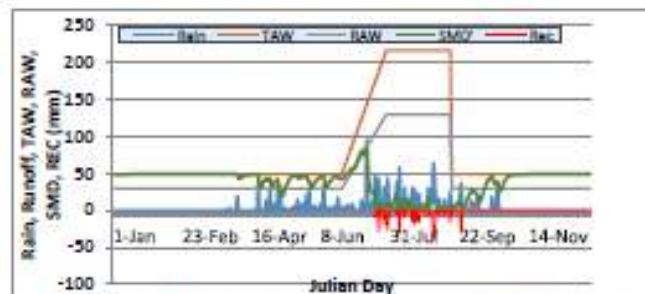
Figure 4: Soil Moisture Balance Components for 2005-Water year
