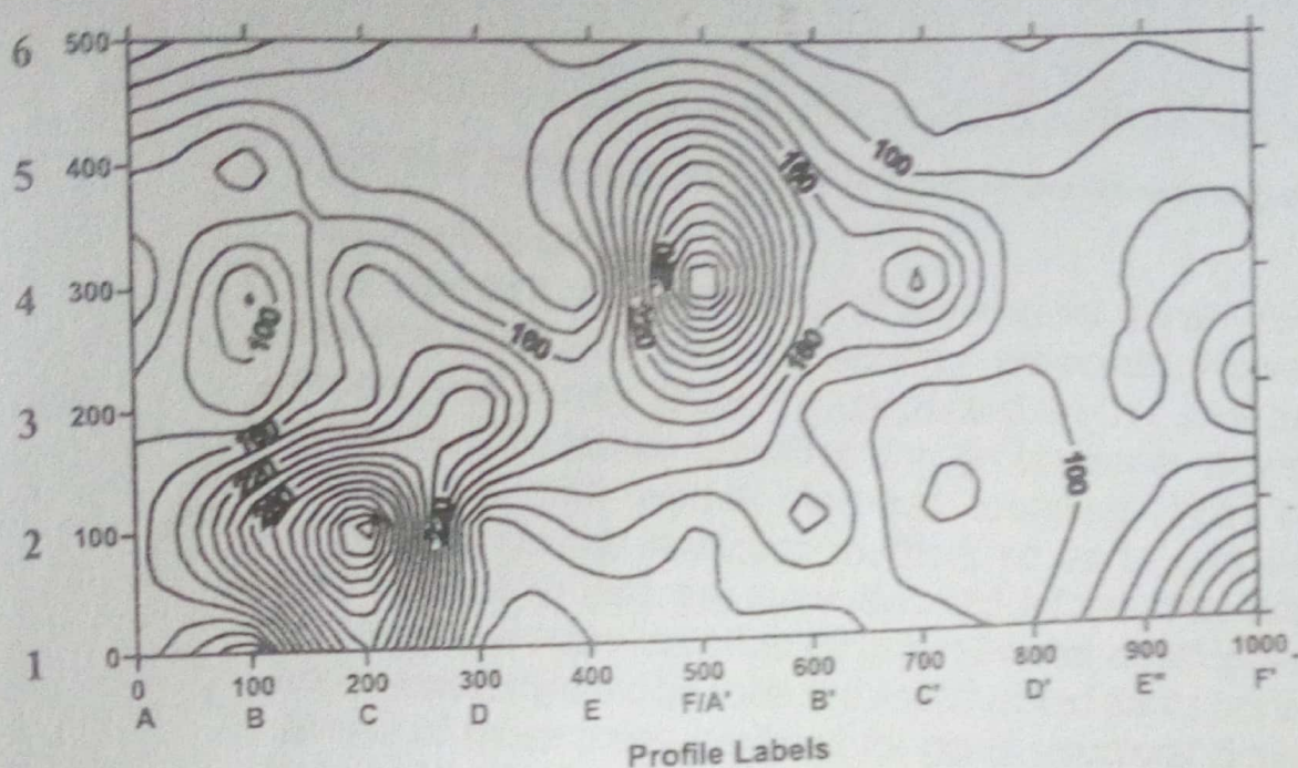
Figure 7: Contour map of Electrical Profiling at 15m Depth (Contour interval is 20Ωm)
