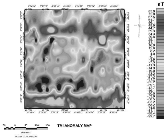
Figure 6: Total Magnetic Anomaly map
