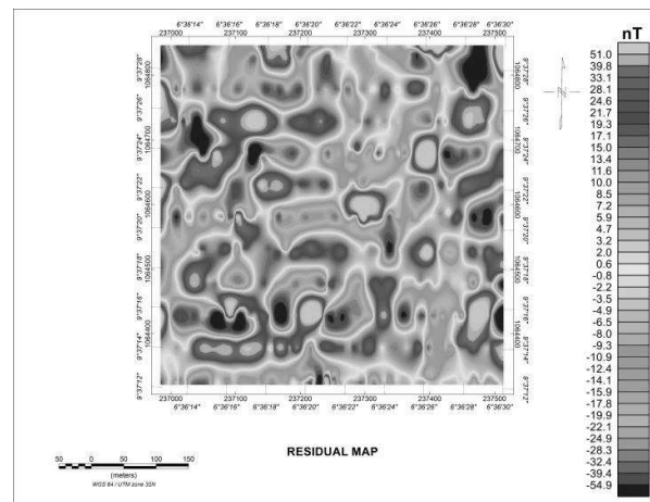
Figure 12: Residual Anomaly Map
