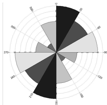
Figure 7: Rose diagram showing fracture and joint direction.
