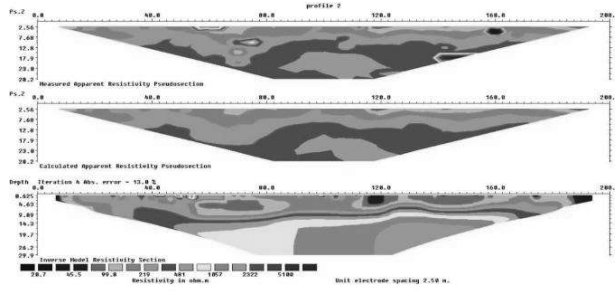
Figure 10: 2-D Resistivity profile on 9° 37' 16.0''N and 6° 36' 28.0''E
