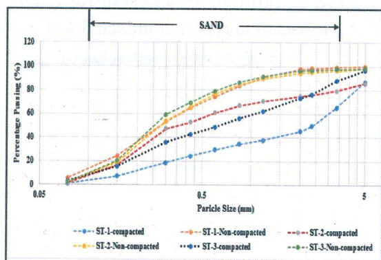
Fig. 2: Particle size distribution of Compacted and Non-compacted soil in all Stations
