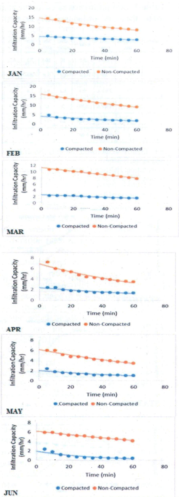
Fig.4: Infiltration rates (Jan-June) for compacted and non-compacted soil for Station 2 (dry& wet season)
