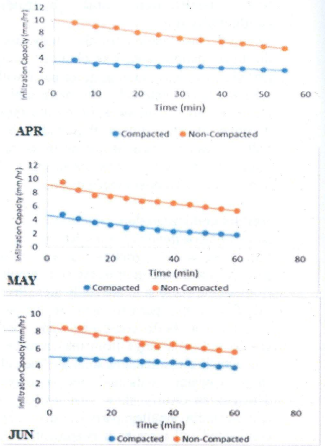
Fig. 3: Infiltration rates (Jan-June) for compacted and non-compacted soil for Station 1 (dry& wet season)
