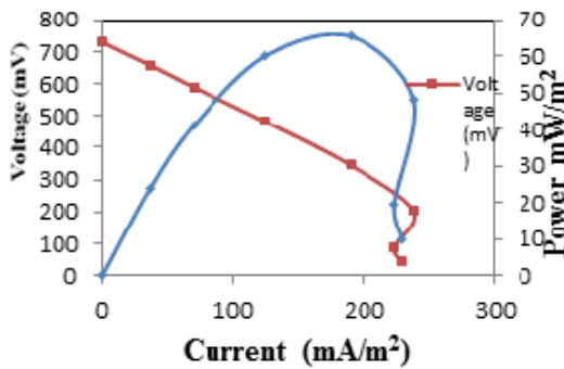
Figure 6. Polarization and Power Density curves of the soil MFC
