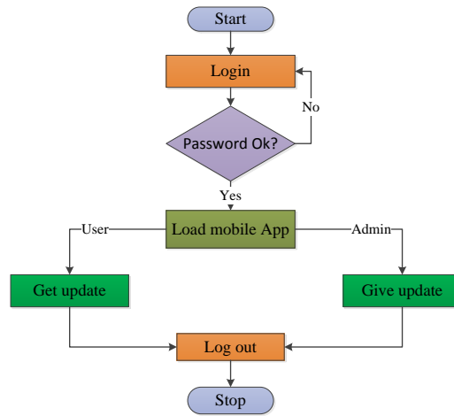
Figure 2. System flowchart
