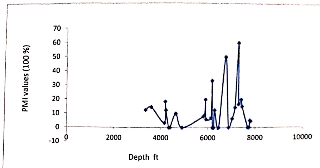
Figure 3 PMI plot for OL-A well
