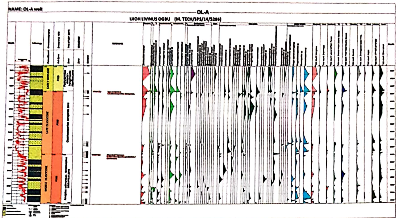
Figure 2 Palynomorph Distribution chart of OL-A well
