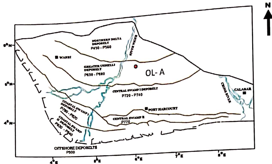
Figure 1 Location of OL-A well, on Greater Ughelli depobelt, Eastern Niger Delta, Nigeria. (Modified after Doust and Omatsola, 1990).
