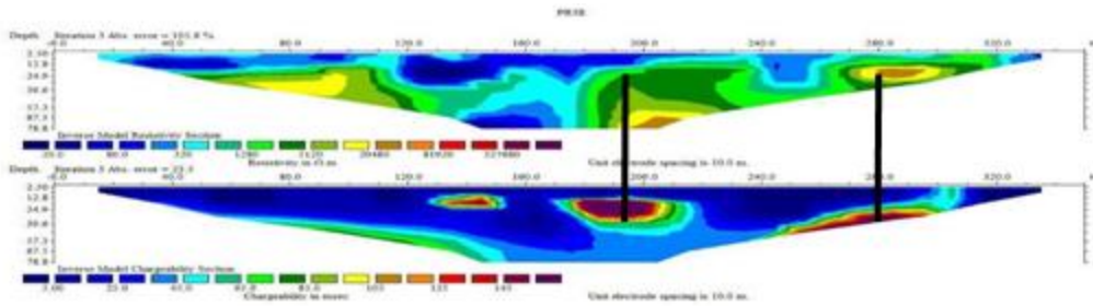
Figure no 12: 2-D inverted IP-Resistivity mode plot for Profile 10B_West (284520 to 284873, 1051600)
