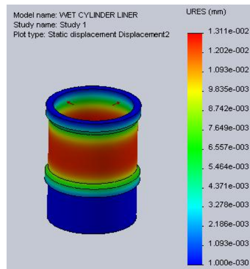
Fig 8: Displacement
