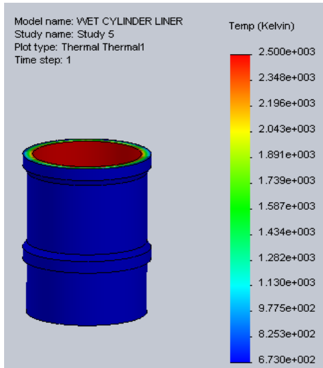
Fig 10: Steady State Thermal Analysis Temperature Distribution
