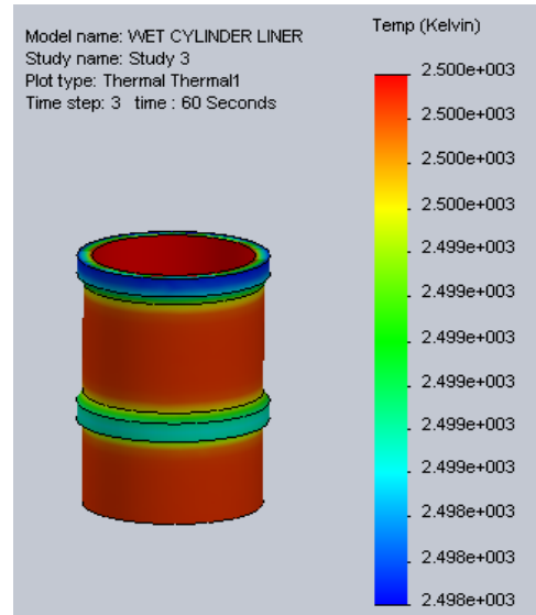
Fig 13: Temperature Distribution after 80 Seconds
