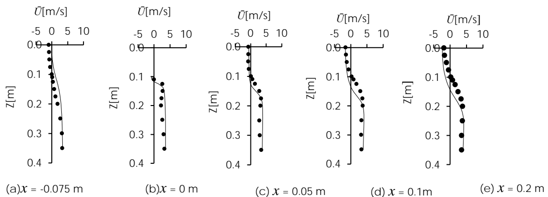
Fig. 9 Profiles of wind tunnel data (dotted points) and simulation results (solid lines) of mean streamwise wind velocity component, \bar{U} , on a horizontal plane at y = 0.0125 m ( \frac{1}{16}h )
