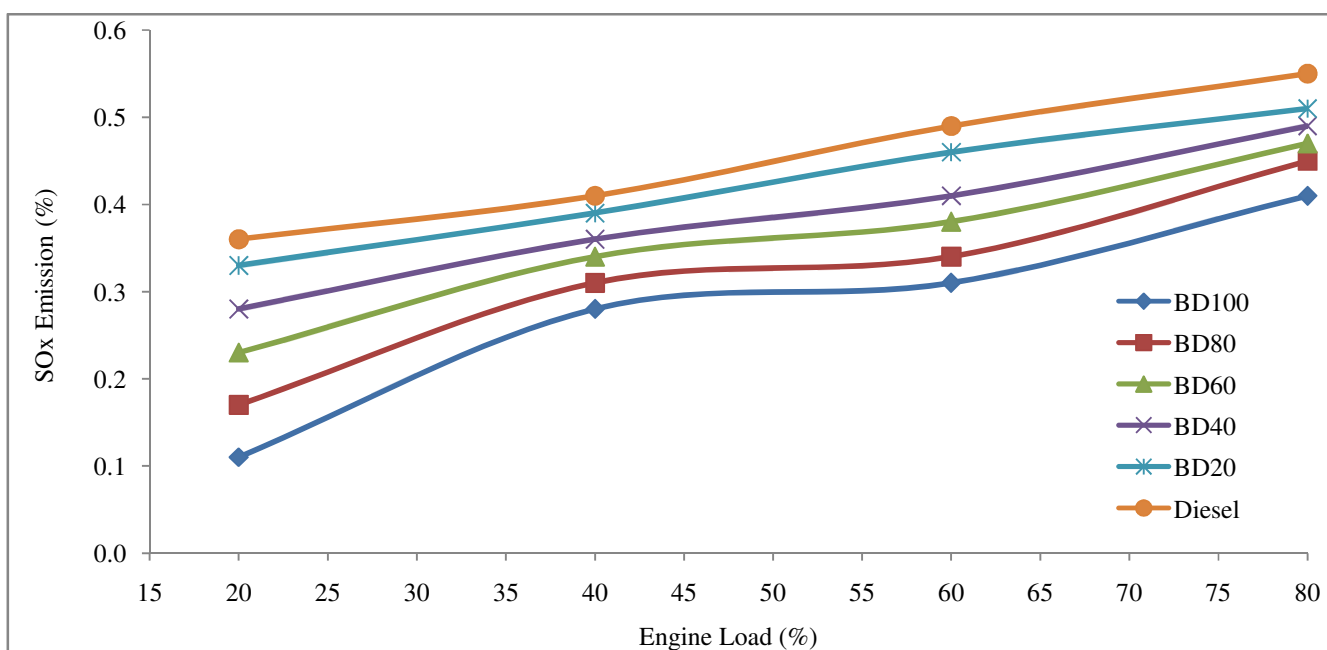
Figure-6: Oxides of Sulphur Emissions against Engine Load.
