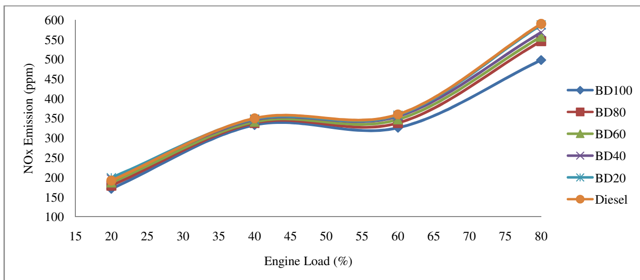
Figure-5: Oxides of Nitrogen Emissions against Engine Load.
