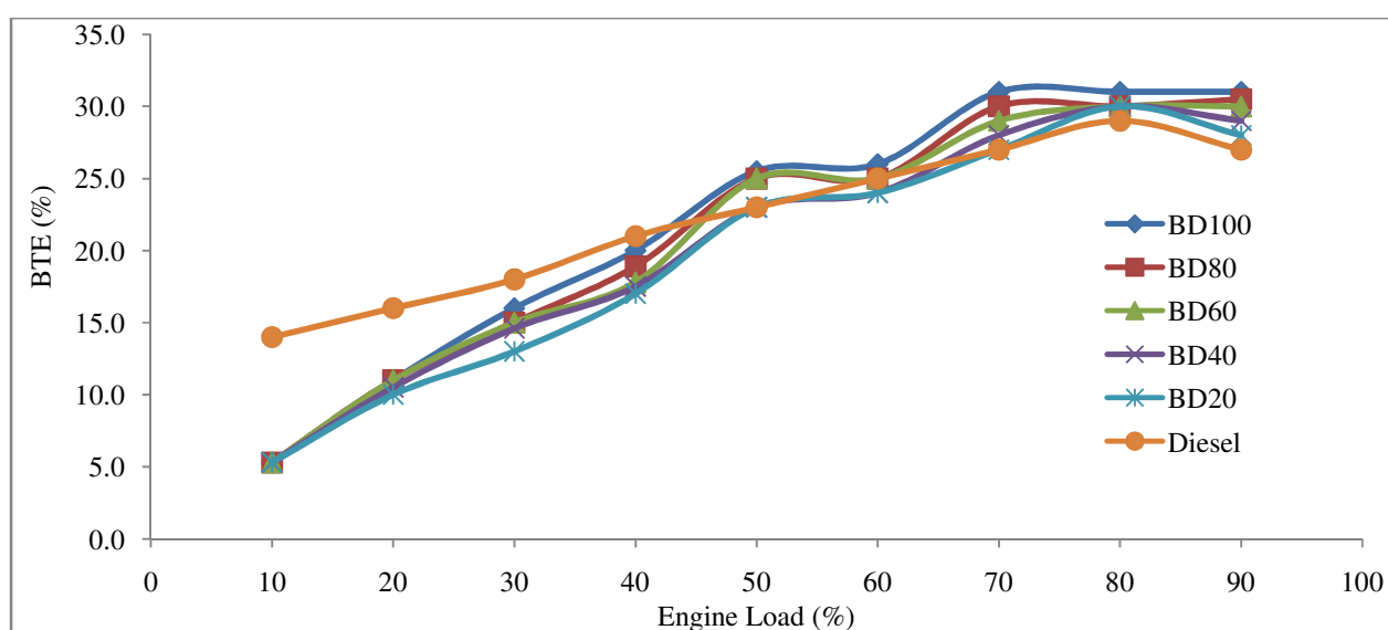
Figure-2: Percentage Brake Thermal Efficiency against Engine Load.
