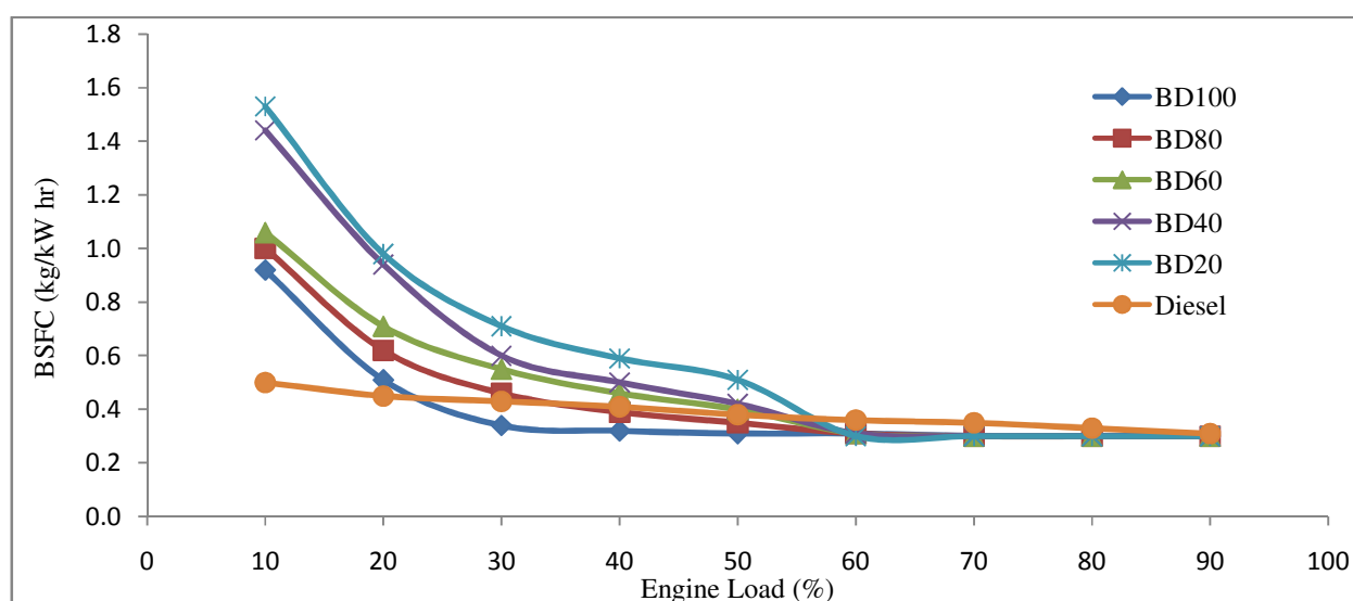
Figure-3: Brake Specific Fuel Consumption Efficiency against Percentage Engine Load.
