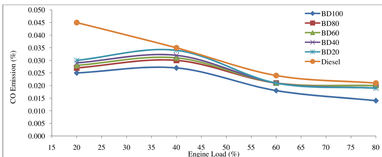
Figure-4: Percentage CO Emission against Engine Load.
