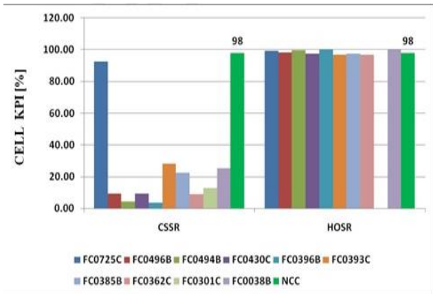
Figure 4: CSSR and HOSR for the Cells during Worst TCH CONG
