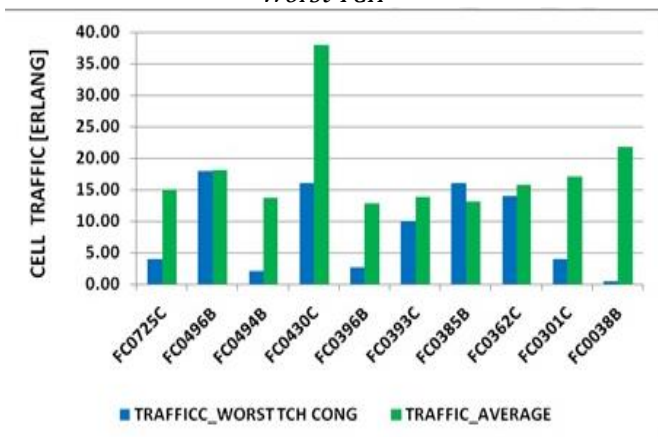
Figure 6: Traffic Average and Traffic Carried by the Cell worst TCH CONG
