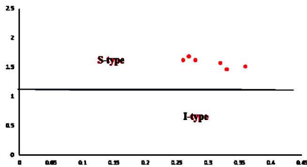
Fig. 10: \text{K}_2\text{O}/\text{Al}_2\text{O}_3 versus \text{Al}_2\text{O}_3/(\text{Na}_2\text{O} + \text{K}_2\text{O} + \text{CaO}) plot for granite samples of study area (after White and Chapell, 1977)
