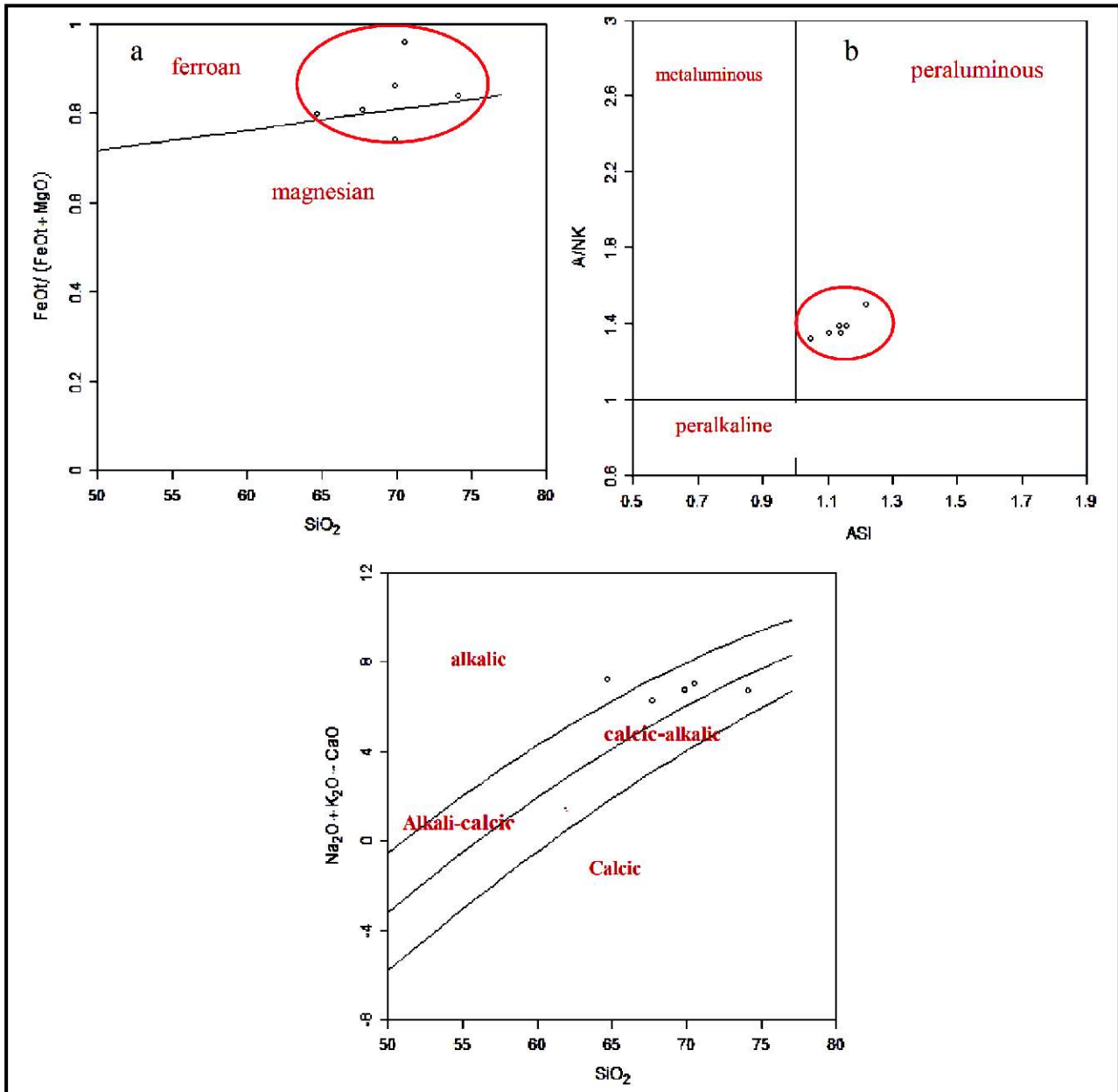
Fig. 9: (a & b): FeOt+MgO against \text{SiO}_2 & A/NK against ASI plot for granite samples of study area (after Frost et al. , 2001) and (c) \text{Na}_2\text{O} + \text{K}_2\text{O} - \text{CaO} against \text{SiO}_2 diagram for granite sample of study area (after Frost et al. , 2001)
