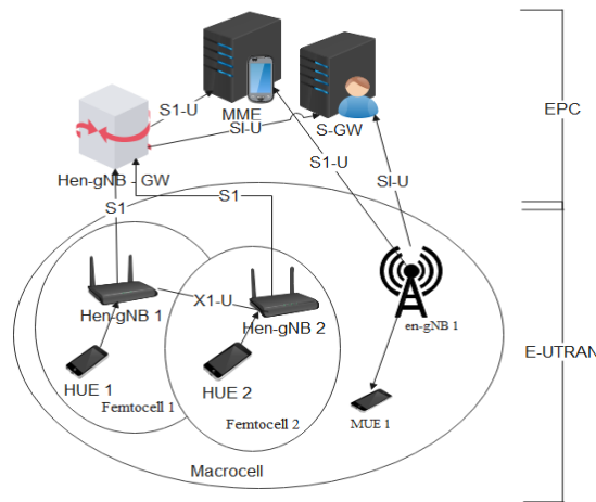
Fig. 1. Schematics of NSA architecture of 5G Macro-Femto HetNet [4–6]
