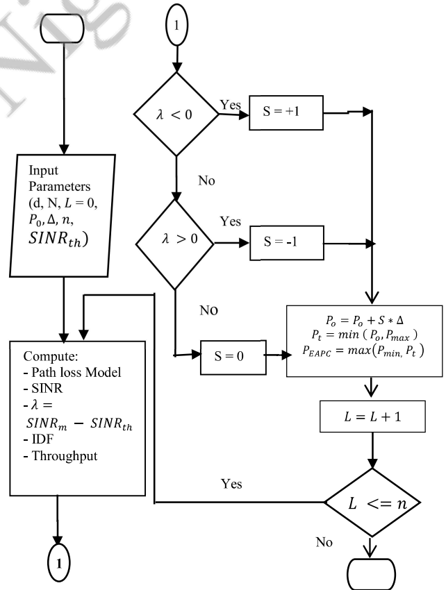
Fig. 2. EAPC flowchart
