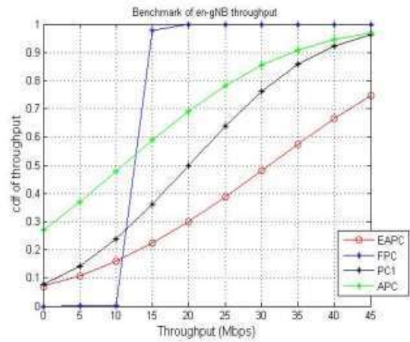
Fig. 6. Benchmark of en-gNB throughput
