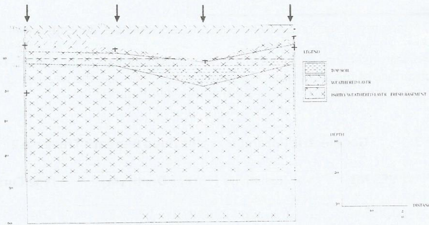
Fig. 9: Geoelectric Section Showing Subsurface Sequences Beneath Traverse3
