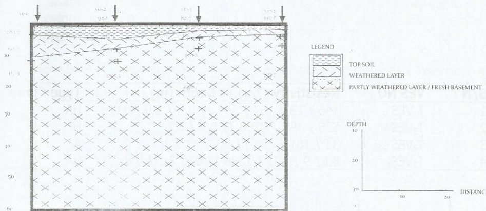
Fig. 7: Geoelectric Section Showing Subsurface Sequences Beneath Traverse1
