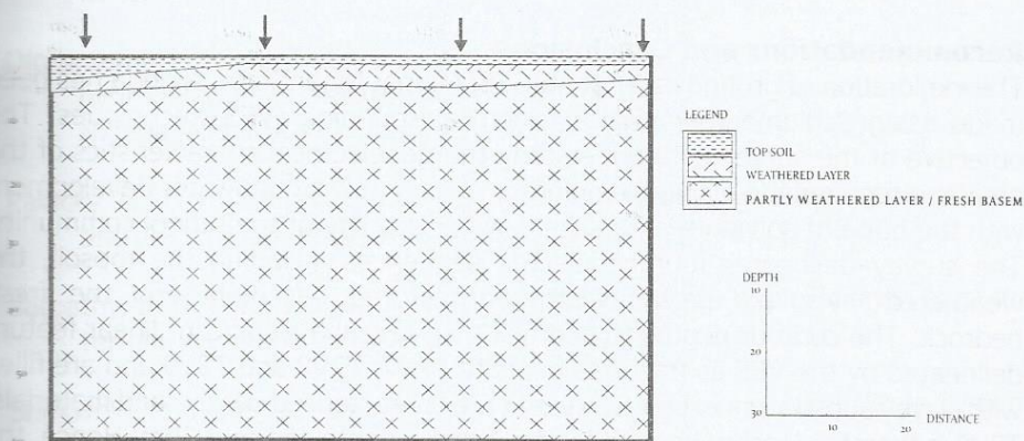
Fig.10: Geoelectric Section Showing Subsurface Sequences Beneath Traverse4
