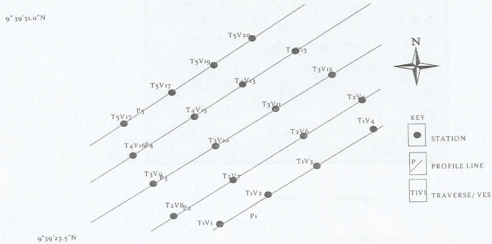
Fig. 3: The VES Data Acquisition Map in the Study Area
