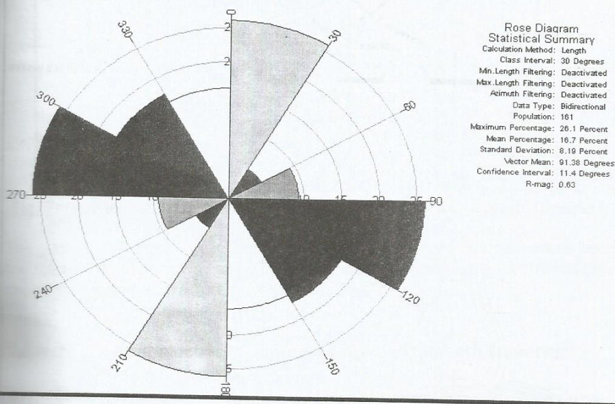
Fig. 4: The Rosette Diagram of the Study Area
