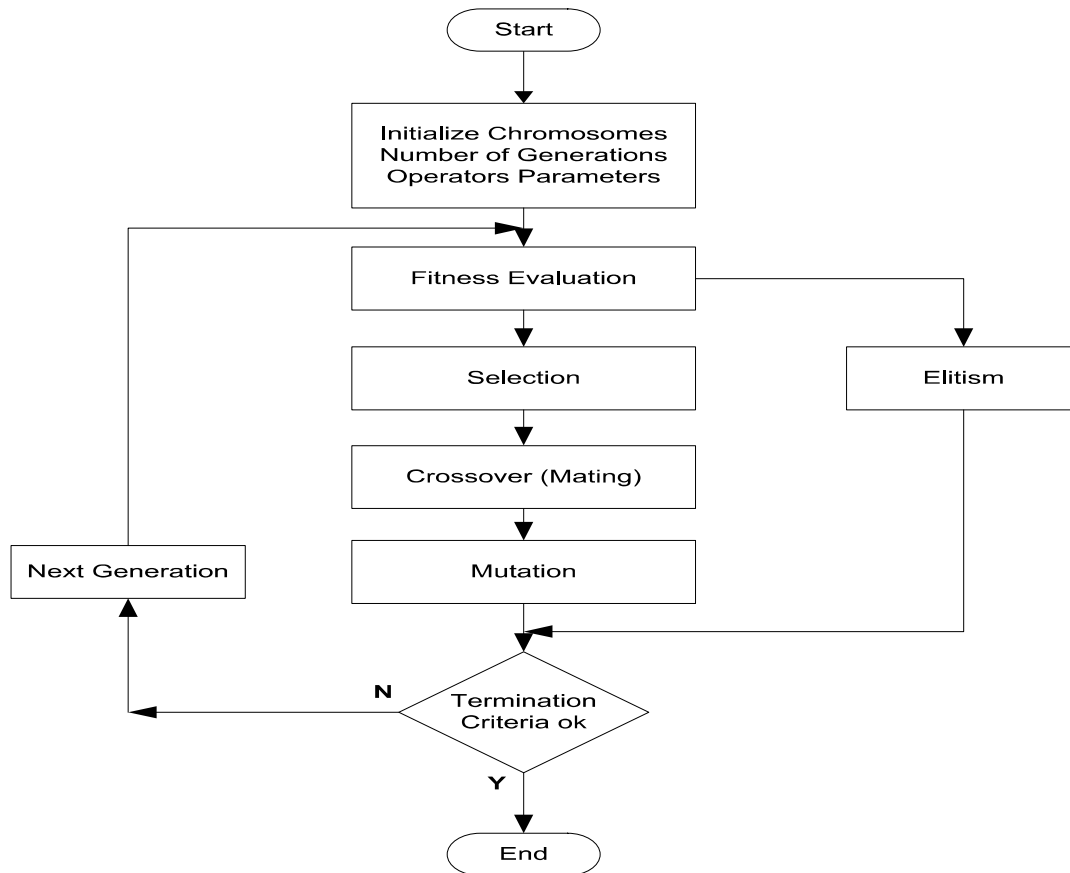
Figure 1: Flowchart of the Timetable Generator
