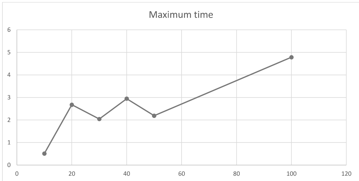
Figure 3: Maximum Time against Population Size
