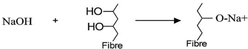
figure 4. chemical surface modification after alkali treatment of kenaf fibers.
