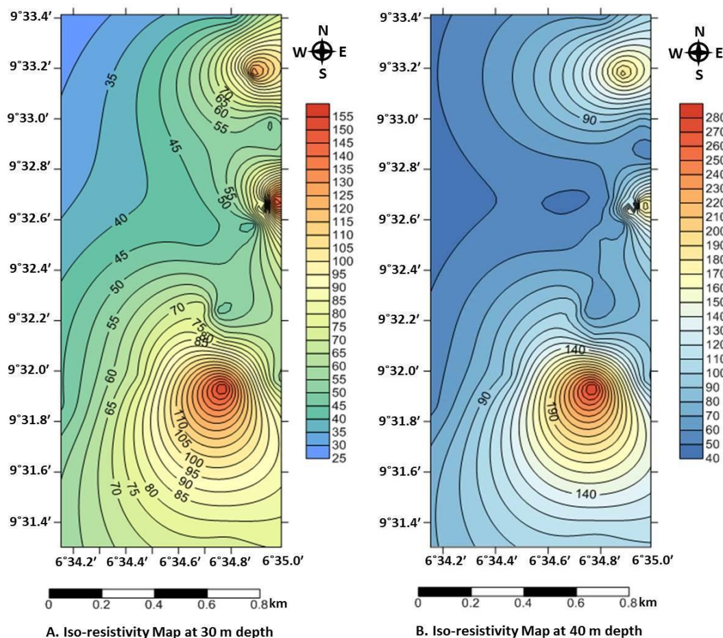
Figure 8: Iso-Resistivity for Vertical Electrical Sounding points 1 – 23 at: A. 30 m depth, and B. 40 m depth.
