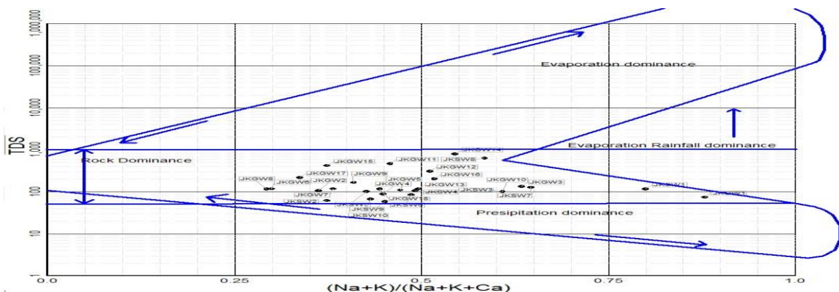
Fig. 5: A representative Gibbs Plot for Hong and Zango communities
