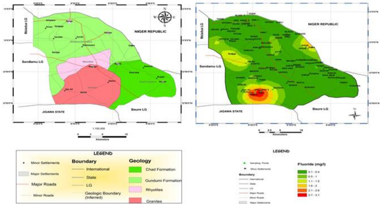
Fig. 3: Comparison of the Geology and Fluoride Concentration in Zango Area
