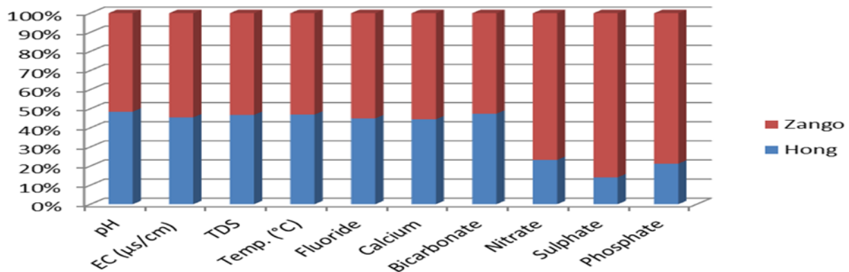
Fig. 4: Comparing the concentration of analyzed parameters in Hong and Zango Communities
