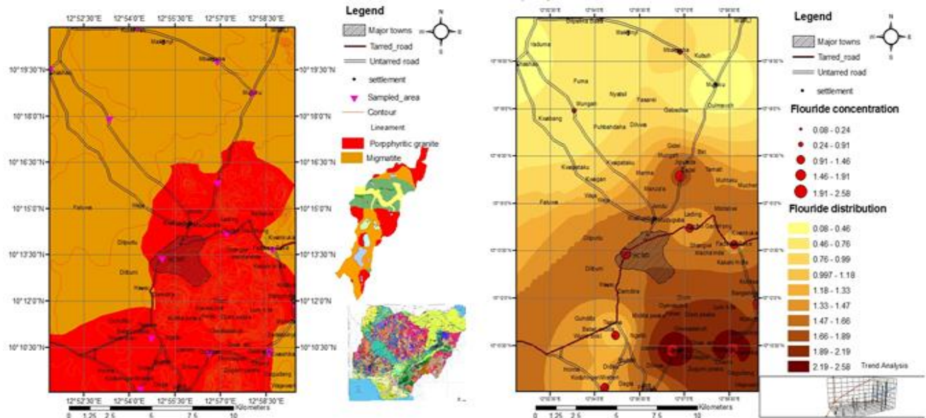
Fig. 2: Comparison of the Geology and Fluoride Concentration in Hong Area
