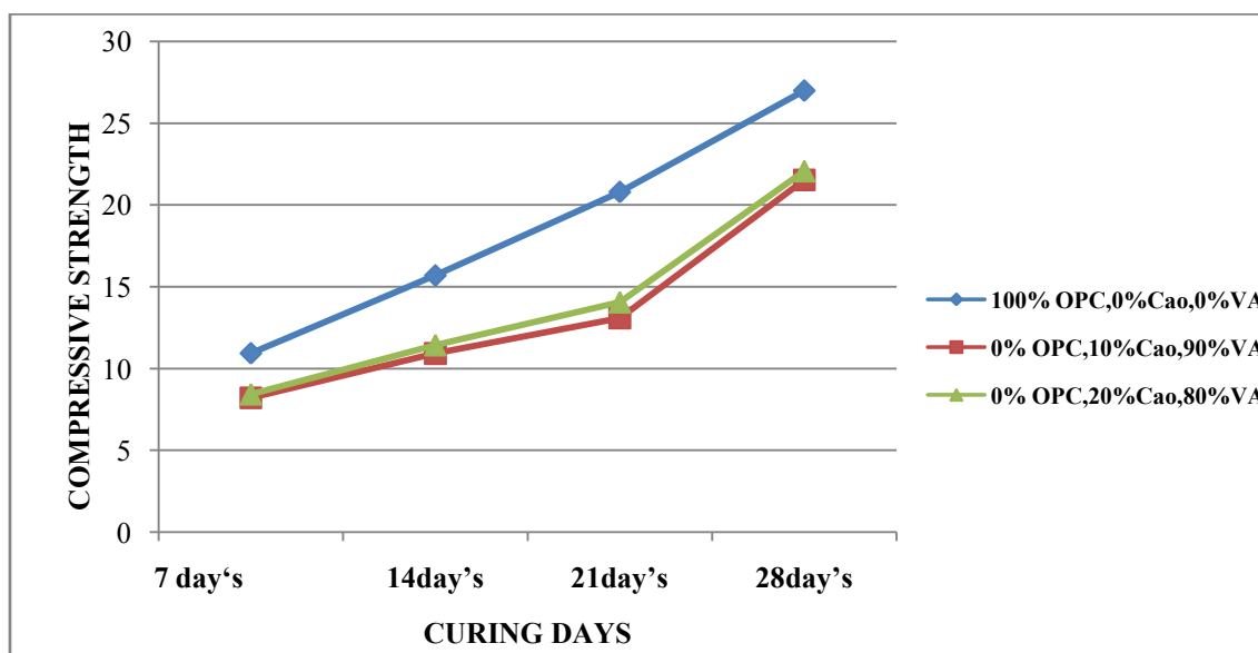
Fig 1: Effect of calcium oxide on performance characteristic of volcanic ash Laterized concrete.
