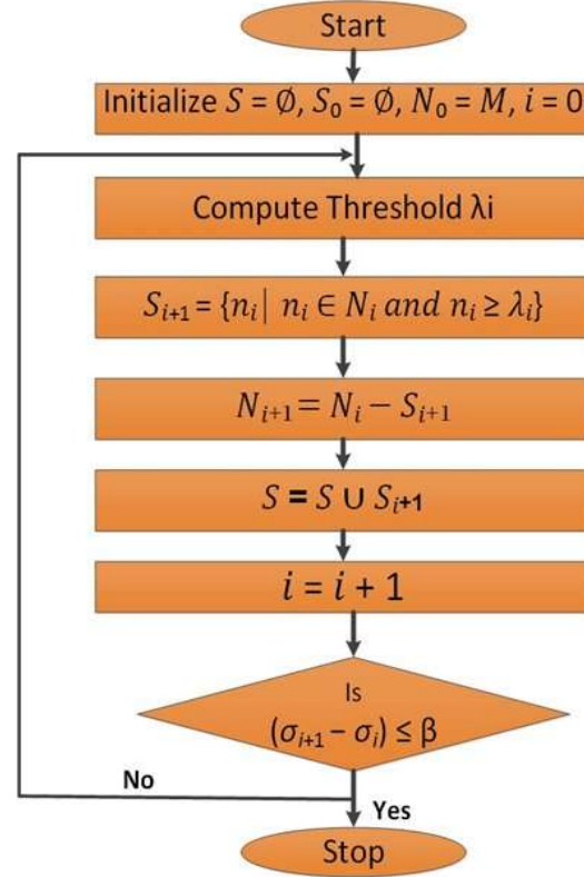
Figure 3: The ROHT Algorithm [11]
