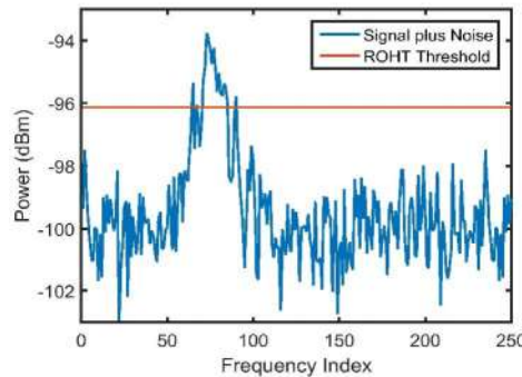
Figure 8: Signal plus Noise spectra at SNR = 5 dB showing the threshold estimated by the ROHT algorithm
