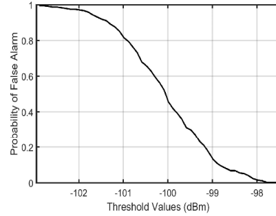
Figure 5: The probability of false alarm computed for the noise only dataset based on a true threshold value of -97 dBm.
