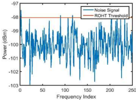
Figure 4: Noise only spectra showing the threshold estimated using the ROHT algorithm
