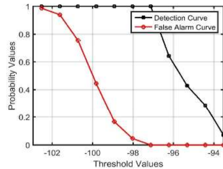
Figure 7: Performance for the Signal plus Noise dataset for (SNR=10dB to 1dB)
