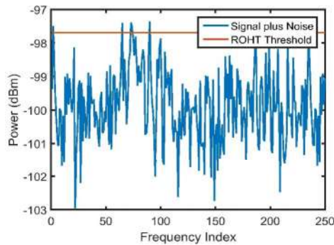
Figure 10: Signal plus Noise spectra at SNR = 1 dB showing the threshold estimated by the ROHT algorithm
