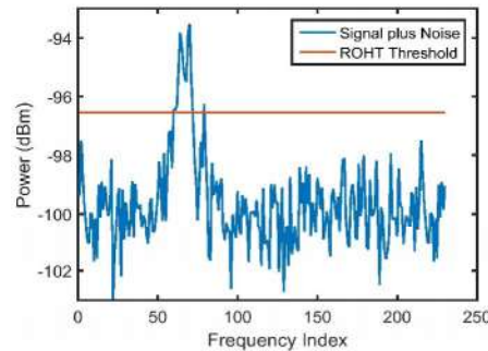
Figure 6: Signal plus noise spectra at SNR = 10dB showing the threshold estimated by the ROHT algorithm
