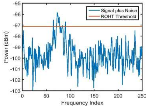
Figure 9: Signal plus Noise Spectra at SNR = 3 dB showing the threshold estimated by the ROHT algorithm
