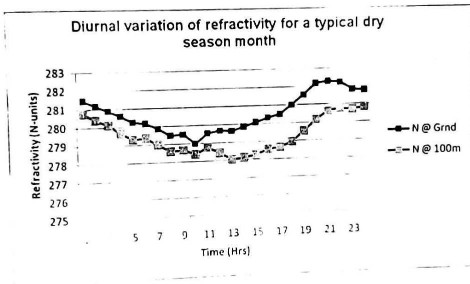
Fig. 1 Mean diurnal variation of N in Minna for a typical dry season month
