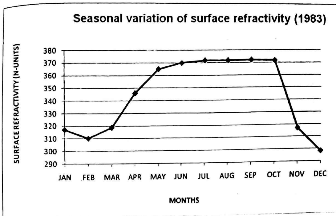
Fig. 4. Seasonal variation of surface refractivity over Minna (1983)
