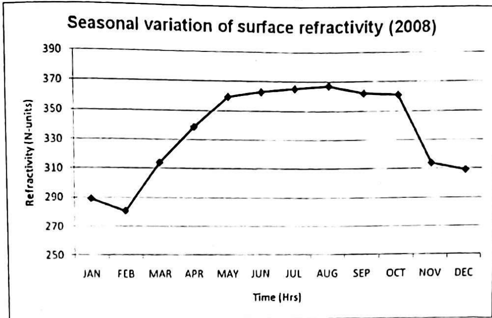
Fig. 3. Seasonal variation of surface refractivity over Minna (2008)
