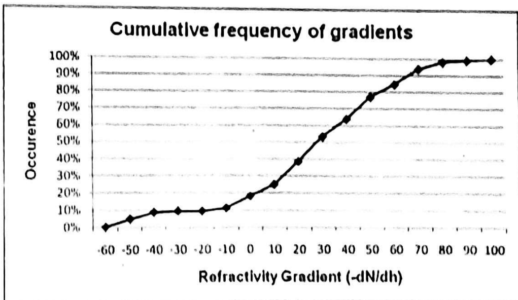
Fig.6. Cumulative frequency of refractivity gradients
