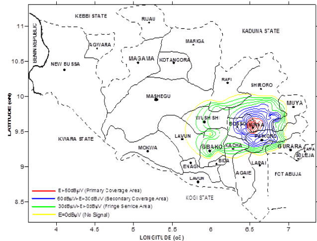
Figure 4. Coverage area of the NTA Minna in Niger State
