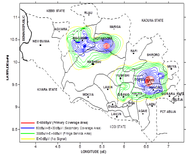
Figure 6. Combined coverage areas of the NTA Minna and NTA Kotangora in Niger State
