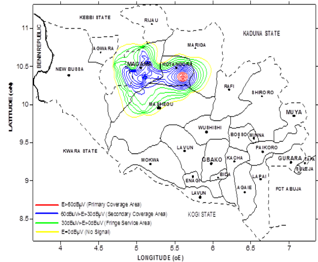
Figure 5. Coverage area of the NTA Kotangora in Niger State
