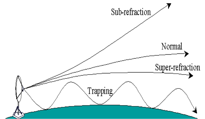
Figure 1. Four classifications of tropospheric refraction [10]
