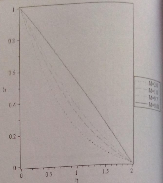
Figure 4. Variation of Hartmann number (M) on h for \alpha=0.6
