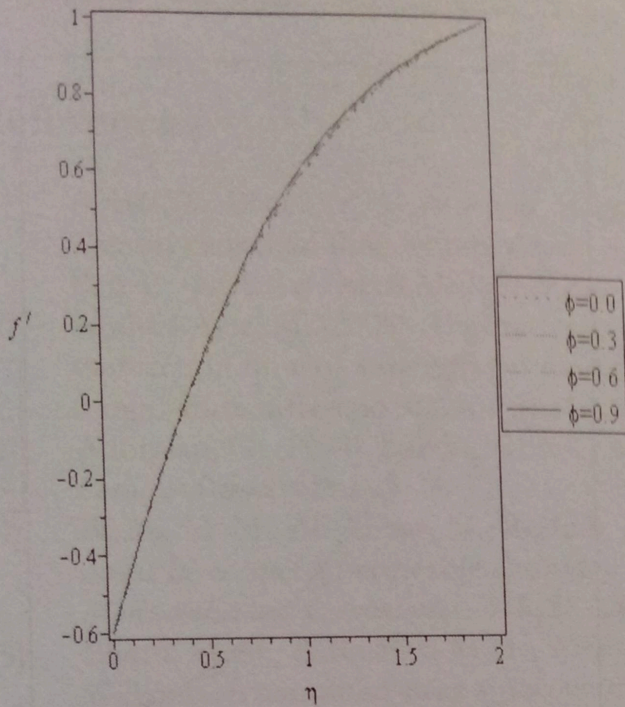
Figure 7. variaon of angle of inclination ( \phi ) on f' for \alpha=-0.6
