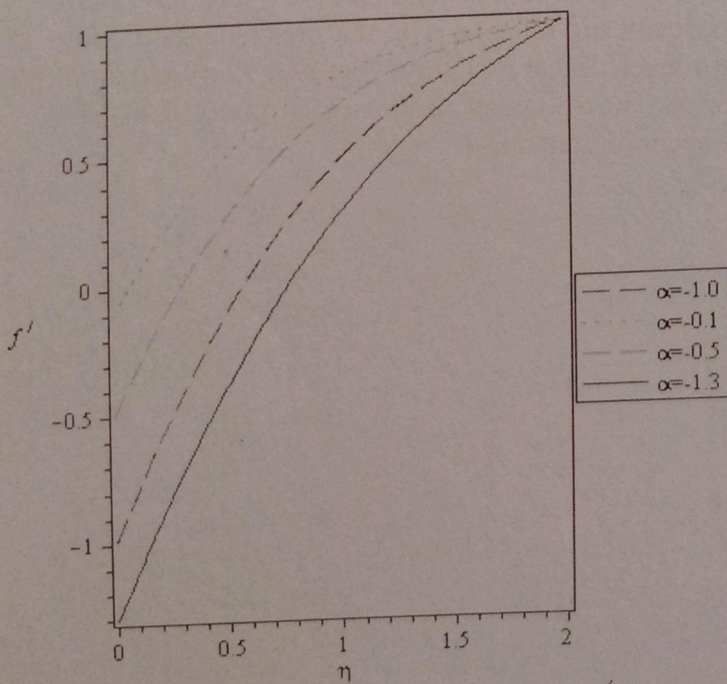
Figure 5. Variation of shrinking parameter ( \alpha ) on f'
