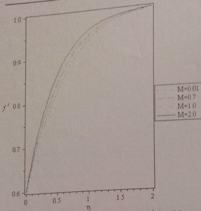
Figure 3. Variation of Hartmann number (M) on f' for \alpha=0.6
