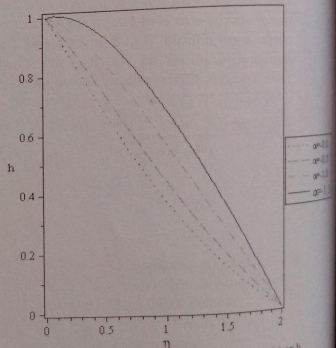
Figure 6. Variation of shrinking parameter ( \alpha ) on h
