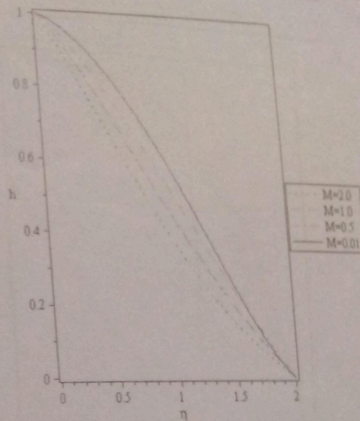
Figure 2: Variation of Hartmann number (M) on h(\eta) for \alpha = 0.6
