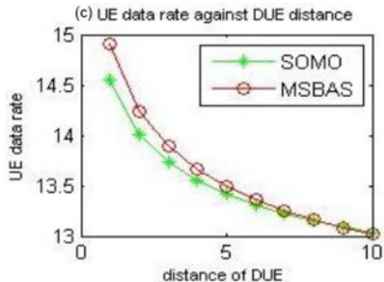
Fig. 8: UE data rate with varied DUE distance.
