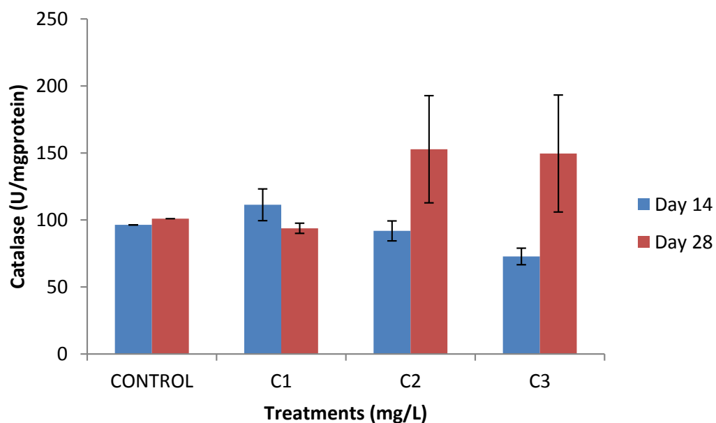
Figure 2. Catalase production level in the gill of C. gariepinus exposed to sub-lethal concentration of lead nitrate.
