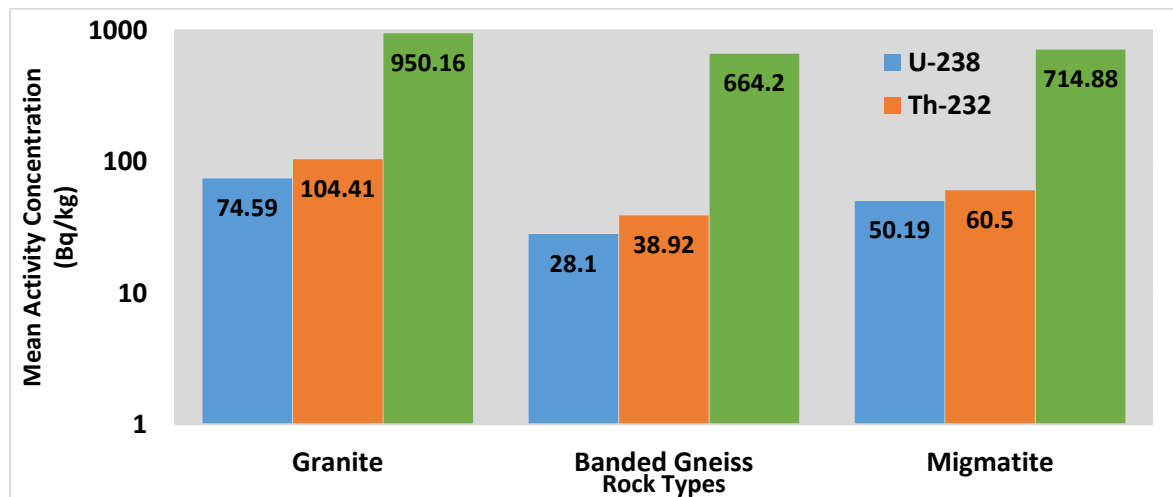
Figure 4. Mean activity concentration of 238 U, 232 Th, and 40 K from rock samples.
