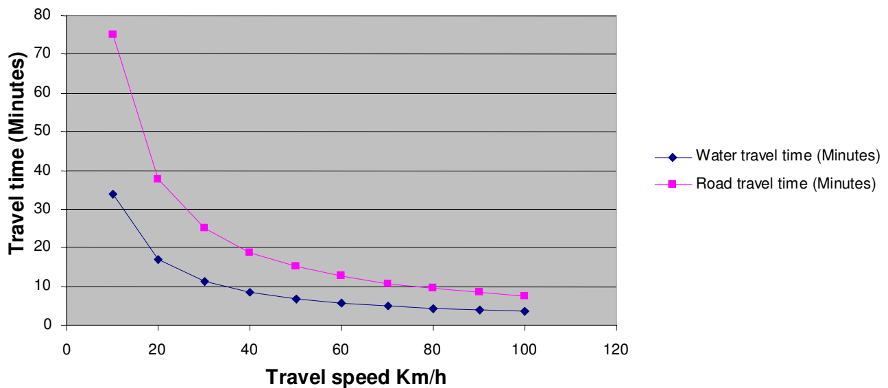
Figure 6. Water travel time at cruise speed, as well as road travel time due to congestion during the peak hours between Victoria Island and Ebute ero.
