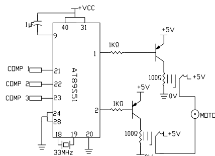
Fig.7. Circuit diagram of the control and relay unit
