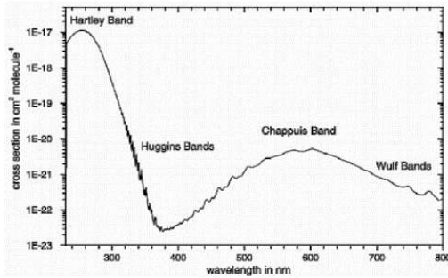
Fig. 4. Ozone Spectrum Showing Absorption Cross Section Versus Wavelength [10]
