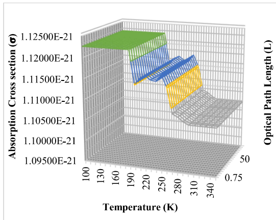
Fig. 2. Simultaneous effects of temperature and optical path-length on OACS at 257.34 nm
