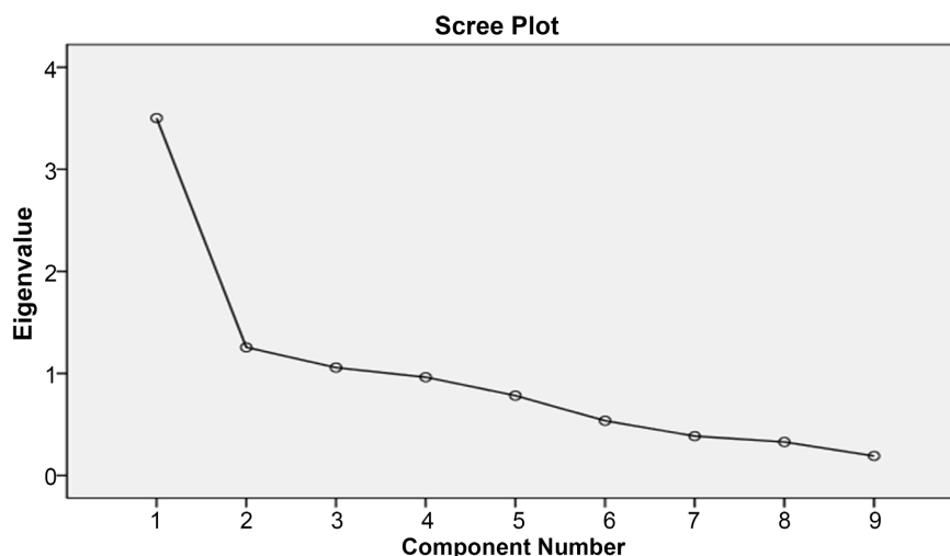
Figure 1. Scree plot.
