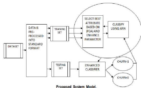
Figure 3: System Model.
