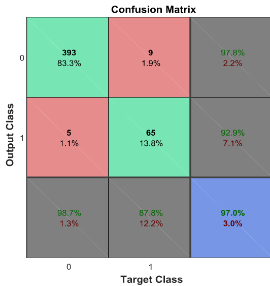
Figure 4: ANN_POA Confusion Matrix
