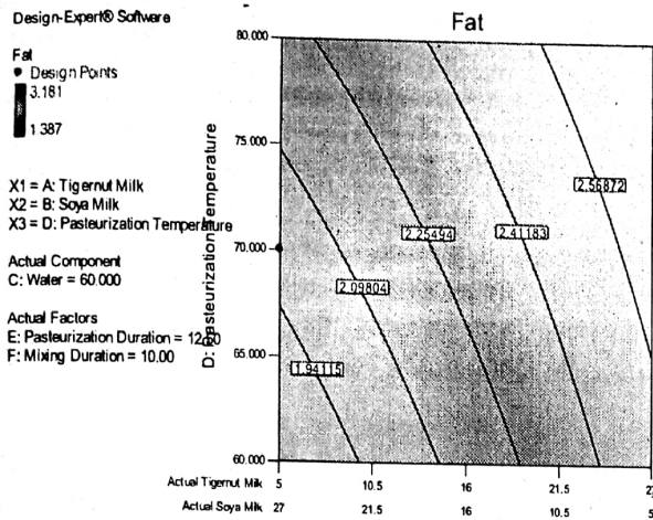
Fig. 7: Contour Mix-Process Plots Showing the Effect of Pasteurization Temperature on Fat Yield
