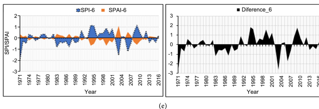
Figure 4. Temporal drought evolution over an annual cycle and change characteristics for selected stations ((a): SPI-3 and SPAI-3 for Kano), ((b): SPI-3 and SPAI-3 for Yelwa), and ((c): SPI-3 and SPAI-3 for month of September in Lokoja), ((d) and (e): 6-month accumulation with difference for Makurdi and Yelwa).
